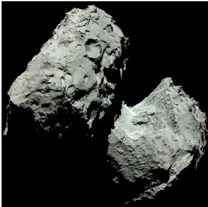
Figure 5 - Close up image of the icy nucleus of the comet 67P/Churyumov-Gerasimenko taken by the ROSETTA probe. Credits: ROSETTA; ESA.
