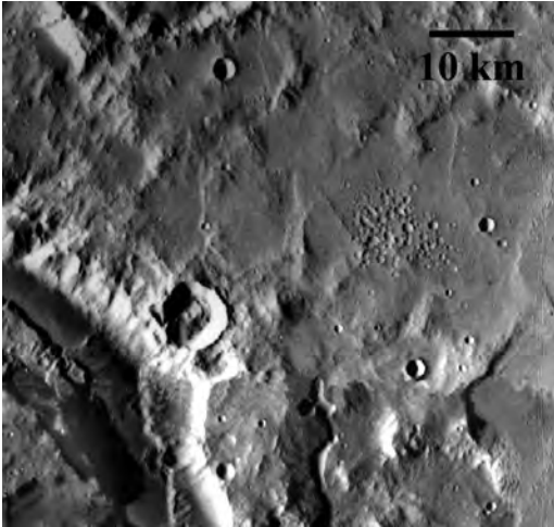
Figure 6 - Viking orbiter image of the Ma'adim Vallis cluster of craters on the surface of planet Mars. Credits: VIKING- NASA
