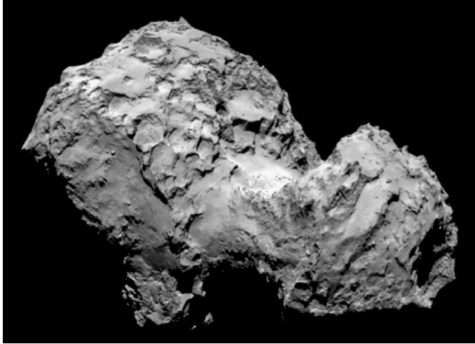
Figure 4 - Image of the icy nucleus of the comet 67P/Churyumov-Gerasimenko taken by the ROSETTA probe. The nucleus is bilobulated (binary) and diameters of the 2 lobes are: Large: 4.10 x 3.52 x 1.63 kilometers; Small: 2.50 x 2.14 x 1.64 kilometers. Credits: ROSETTA; ESA.
