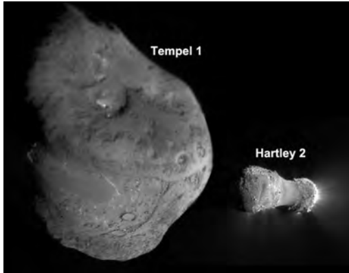
Figure 3 - Image showing the icy nuclei of the comets 9P/Tempel 1 and 103P/Hartley 2 at the same scale. Both objects have extremely dark albedos. The nuclei sizes are: 9P/Tempel 1: 7.5 x 5.0 Kilometers; 103P/Hartley 2: 2.2 x 1.5 Kilometers. Credits: NASA.
