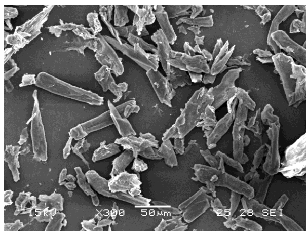
Fig. 4. FESEM micrograph of CMF.
