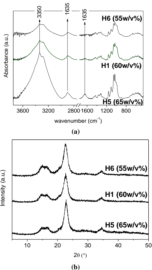
Fig. 10. Effect of acid concentration on the FTIR (a) and XRD (b) spectra of CNF (temperature: 45°C, time: 25min.).
