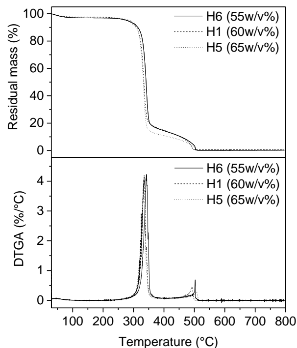
Fig. 11. Effect of acid concentration on the TGA and DTGA curves of CNF (temperature: 45°C, time: 25min.).
