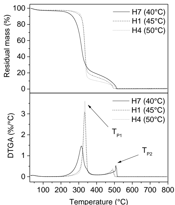
Fig. 6. Effect of reaction temperature on the TGA and DTGA curves of CNF (time: 25min., acid concentration: 60w/v%).
