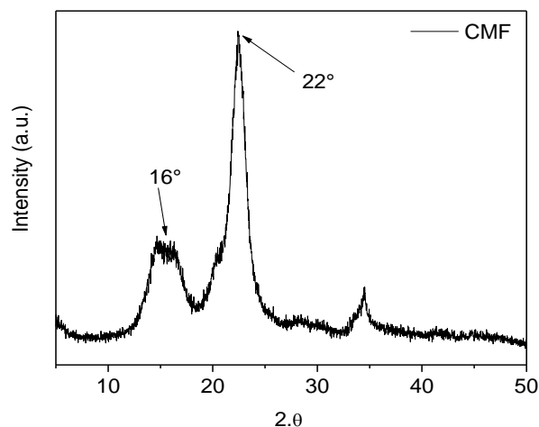
Fig. 2. XRD curve of cellulose microfibrils.
