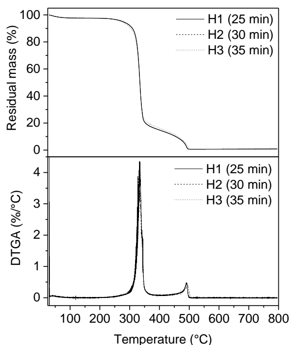
Fig. 9. Effect of reaction time on the TGA and DTGA curves of CNF (temperature: 45°C, acid concentration: 60w/v%).
