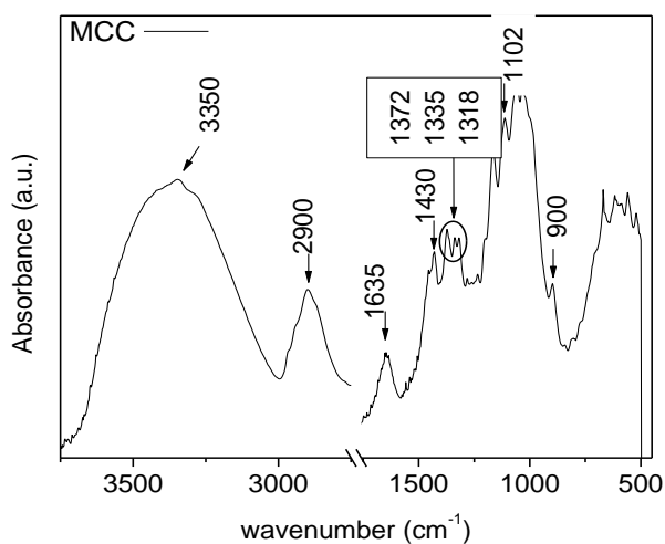
Fig. 1. FTIR spectra of cellulose microfibrils.
