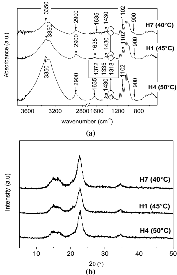
Fig. 5. Effect of reaction temperature on the FTIR (a) and XRD (b) spectra of CNF (time: 25min., acid concentration: 60w/v%).
