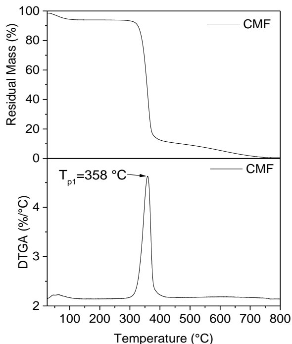
Fig. 3. TGA and DTGA curves of cellulose microfibrils.
