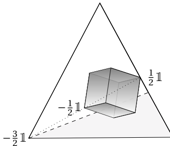
FIGURE 3. The simplex S(-\frac{3}{2}\mathbb{1}, 3e_1 - \frac{1}{2}\mathbb{1}, 3e_2 - \frac{1}{2}\mathbb{1}, 3e_3 - \frac{1}{2}\mathbb{1}) enclosing the cube [-\frac{1}{2}, \frac{1}{2}]^3 \subset \mathbb{R}^3 as in Example 3.1.
