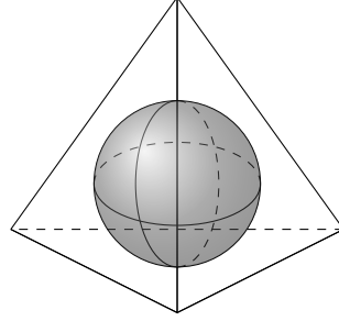
FIGURE 2. The simplex of minimal volume enclosing the Euclidean ball is the regular simplex circumscribing it.
