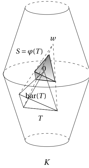
FIGURE 1. Construction involved in the proof of Theorem 1.5.
