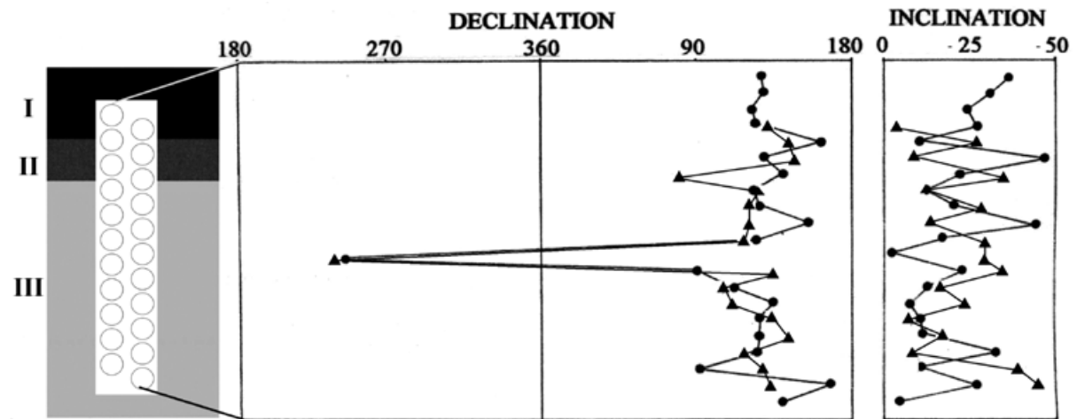
Figure 10. Overlapped stratigraphic display of ET1 and ET2 logs respectively represented by solid circles and triangles related with the direct absolute date by 14C. Roman numerals to the left indicates the geological layers.
