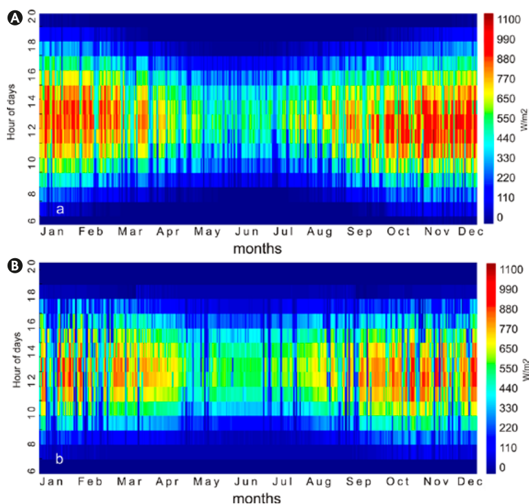
Figure 2. Annual horizontal global radiation mapping ( \text{W/m}^2 ). Mendoza city (A) and Campinas (B).
