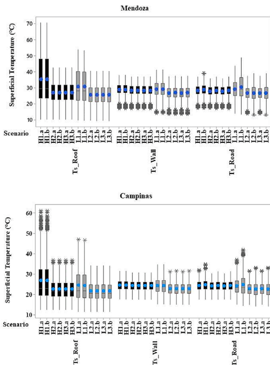
Figure 5. Box plot diagram of surface temperatures in the both cities studied. Black columns indicate high H/W scenarios and gray columns indicate low H/W scenarios. a. Mendoza city. b. Campinas city.
