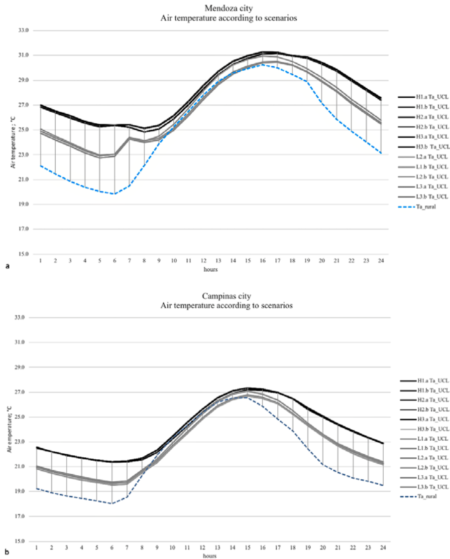
Figure 4. Air temperature curves of Mendoza scenarios ( Ta_{UCL} ) according to albedo level percentage of vegetation and H/W. a. Mendoza city. b. Campinas city.
