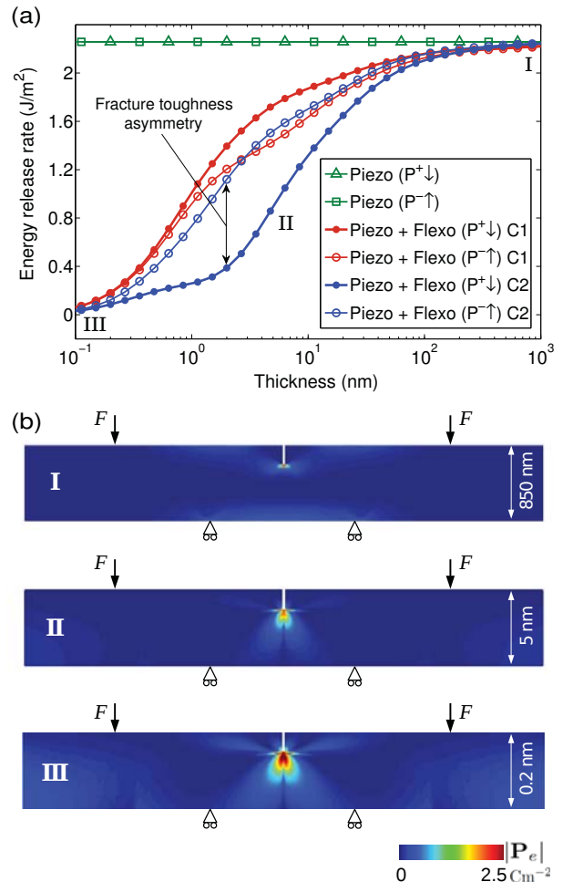
FIG. 2. (a) Energy release rate as a function of the thickness of the poled piezoelectric beam with and without flexoelectricity. The results are obtained considering the material is poled parallel (+) and anti-parallel (-) to the crack. Two cases of the flexoelectric coefficients (C1: \mu_{11} = \mu_{12} and C2: \mu_{12} = -10\mu_{11} ) are considered for the piezoelectric beam with flexoelectricity. (b) Distribution of the polarization magnitude |\mathbf{P}_e| for three different thicknesses (marked as I - III above) considering the positively poled piezoelectric beam with flexoelectricity in the C2 case.
