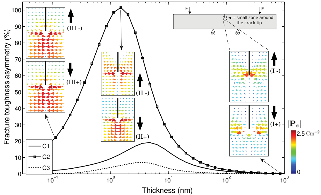
FIG. 3. Fracture toughness asymmetry as a function of the beam thickness. The asymmetry is obtained as the absolute percentage difference between the energy release rates of the negatively and positively poled piezoelectric beams with flexoelectricity, presented in Fig. 2 for two cases of the flexoelectric coefficients (C1: \mu_{11} = \mu_{12} and C2: \mu_{12} = -10\mu_{11} ), and the additional case C3: \mu_{11} = 2\mu_{12} . The insets show the distribution of the polarization \mathbf{P}_e in a small zone around the crack tip at three different length-scales for the negative (top) and positive (bottom) poling directions in the C2 case. The bold black line shows the position of the pre-crack and the bold black arrow indicates the poling direction of the beam.
