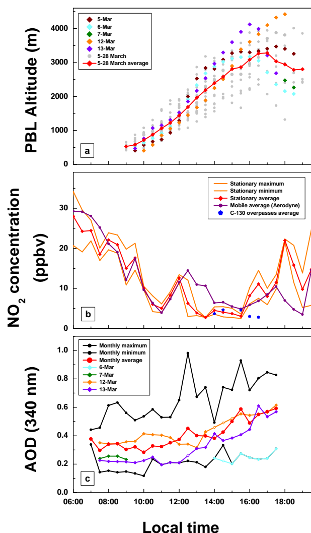
Fig. 1. Diurnal variation at T1 site of (a) PBL altitude above ground (a.g.l.) (color symbols correspond to the cloudless days); (b) NO 2 concentration measured by a stationary instrument (6–31 March), a co-located Aerodyne mobile laboratory (19–22 March), and from the C-130 aircraft overpasses (8, 10, 18, 22, and 29 March); (c) aerosol optical depth at 340 nm (AERONET, 6–31 March) (open symbols correspond to interpolations).
