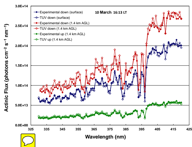
Fig. 6. Spectral variation of the measured and calculated actinic flux at surface and at 1.4 km (a.g.l.) (downwelling and upwelling) for 10 March 2006 at 16:13 local time. PBL altitude at this moment was 3 km (a.g.l.).
