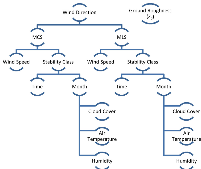
Fig. 1. Tree of decisions based pre-processing operations of meteorological databases. MLS: most likely scenario; MCS: the most conservative scenario.
