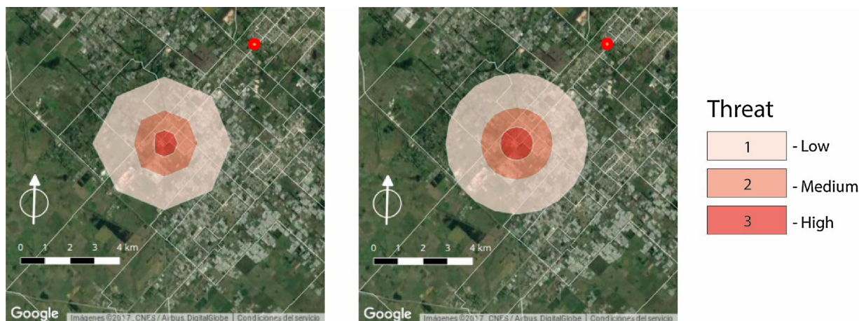
Fig. 6. Toxic threat zones constructed with QGIS from the graphical outputs of ALOHA (composition of 8 directions). On the left, the toxic threat zone of MLS. On the right, the toxic threat zone of MCS. Red point: Interzonal Hospital Specialized in Acute and Chronic Neuropsychiatric "Dr. Alejandro Korn" (For interpretation of the references to colour in this figure legend, the reader is referred to the web version of this article).
