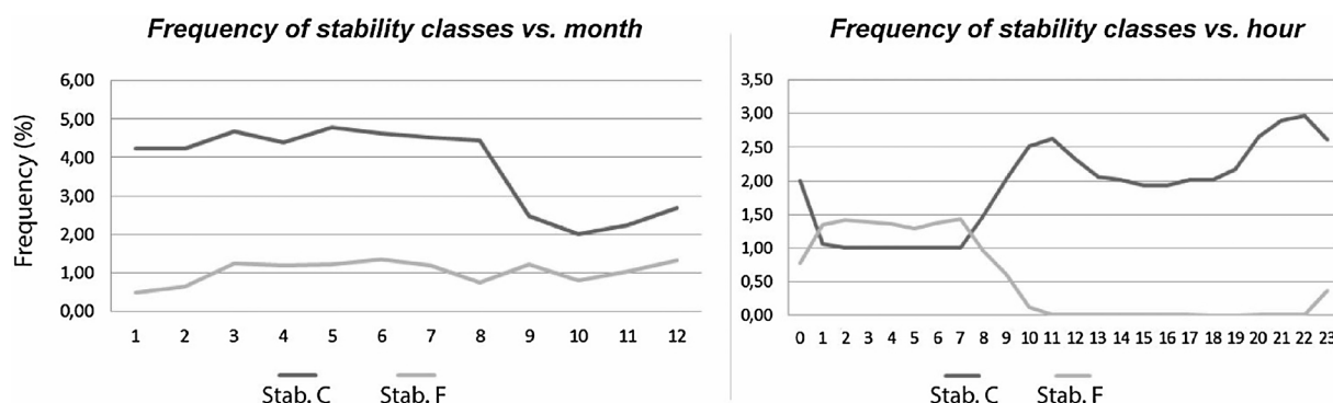
Fig. 5. On the left, the graph shows the frequency of C and F stability classes as a function of the month for the period 2014–2016. On the right, the graph shows the frequency of C and F stability class as a function of the hour for the same period.
