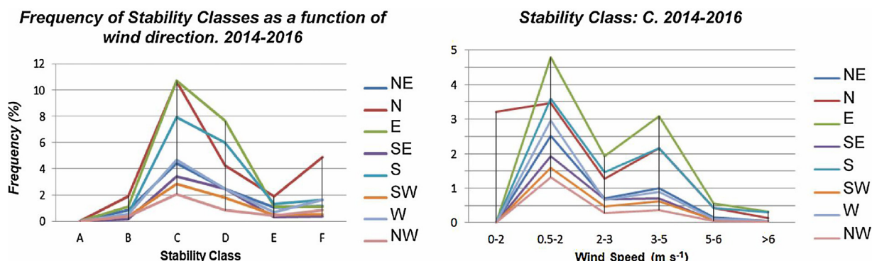
Fig. 4. On the left, the graph shows the frequency of stability classes as a function of wind direction for the period 2014–2016. On the right, the graph shows the frequency of stability class C as a function of wind speed for the same period.
