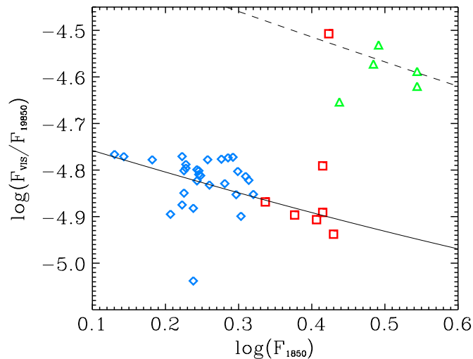
Figure 9. Ratio of the visual flux, F_{\text{VIS}} converted from the IUE FES magnitudes and F_{1850} from Table 2, plotted against F_{1850} . Small open squares—data before 1994; triangles—data of 1994; large squares—data after 1995 January. The continuous line corresponds to the relation of F_{\text{VIS}}/F_{1850} vs. F_{1850} for a blackbody energy distribution flux of different temperatures assuming a constant luminosity. The dashed line is the same relation but with a luminosity that is six times larger, implying that the 1994 eruption involved a significant change in the luminosity.
