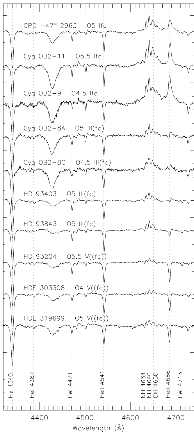
Figure 1. Luminosity sequence of Ofc spectra in the blue–green region. The ordinate is rectified intensity and the longer tick marks are separated by 0.5 continuum units. In addition to the stellar lines identified, the unidentified diffuse interstellar bands at \lambda\lambda 4430, 4502, 4726 are prominent.
