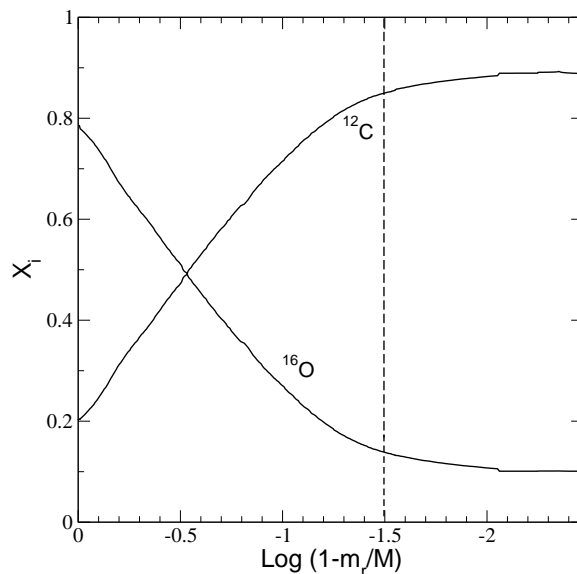
Figure 2. Chemical profile the WD of Fig. 1 when the core is 95% crystallized. Shown is the composition from the center of the WD to 10^{-3} M from its surface as a function of \log(1 - m_r/M) . Here m_r is the mass inner to radius r and M is the total mass of the WD. The vertical dashed line shows the mass coordinate at which the carbon mass abundance is largely enhanced by crystallization ( X_{\text{C}} \gtrsim 0.85 ).
