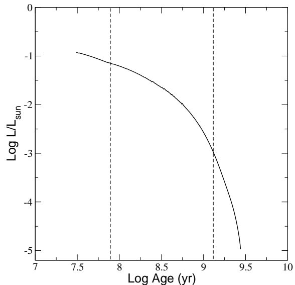
Figure 1. Cooling sequence of the bare nucleus of a 1.38 M_{\odot} carbon-oxygen WD. The leftmost dashed vertical line shows when crystallization starts at the centre of the star, while the rightmost marks when the core is 95% crystallized.
