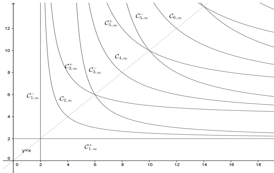
Figure 3. \Sigma_\infty for the unit interval in \mathbf{R} .
