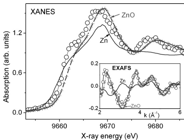
Fig. 3. X-ray absorption near the Zn K-edge (XANES) spectrum obtained for a ZnO NW sample deposited at T_s = 700^\circ\text{C} (circles). The reference spectra for a ZnO crystal (crosses and dash-dot line) and metallic Zn (solid line) are also shown for comparison. Inset: Corresponding extended X-ray absorption fine structure (EXAFS) spectrum, together with the corresponding ZnO and Zn reference spectra.
