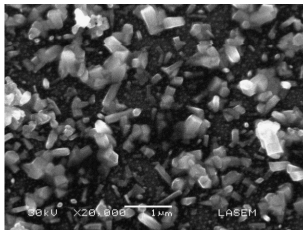
Fig. 4. ZnO structures grown on a (100) Si substrate dispersed with Au catalysts under the same deposition conditions as the sample shown in Fig. 1(a and c).
