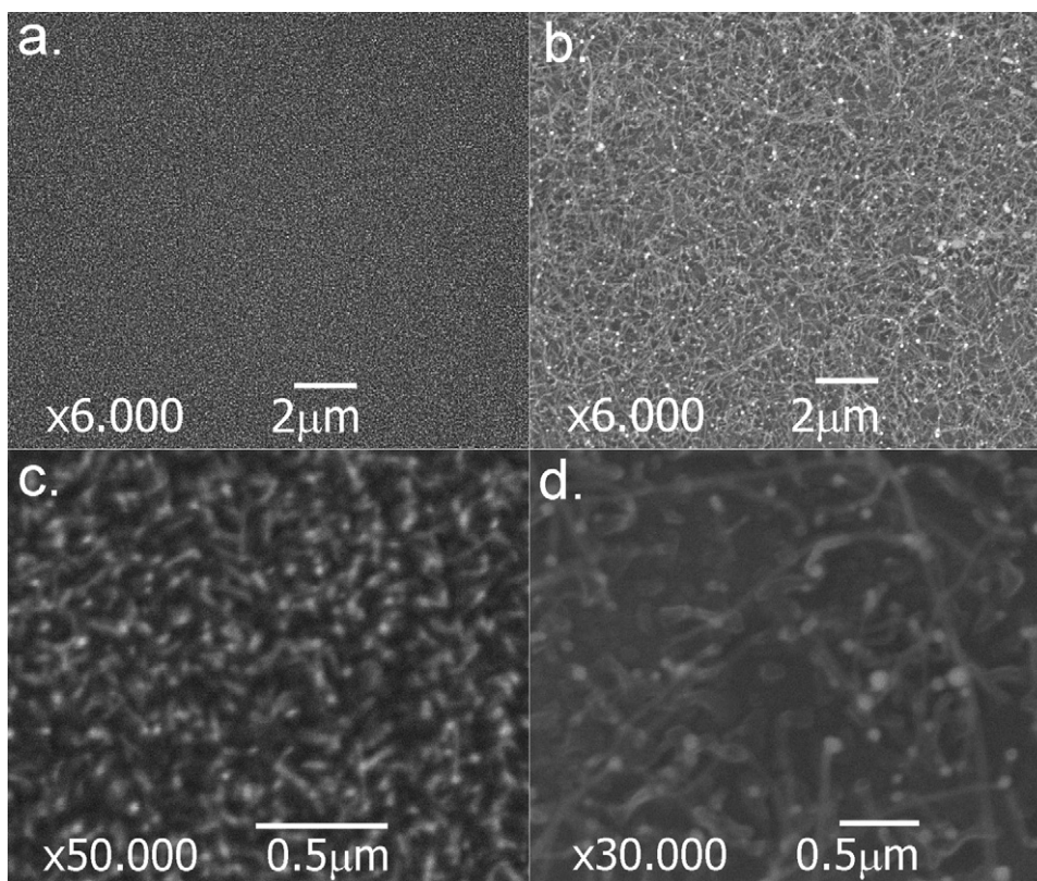
Fig. 1. SEM images under different magnifications of ZnO NWs deposited on Au catalyst/SiO 2 substrate. Left (a and c) correspond to T_s = 520^\circ\text{C} and right (b and d) to T_s = 700^\circ\text{C} .
