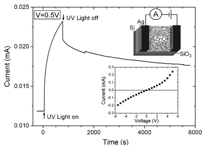
Fig. 5. Electrical current as a function of time for ZnO NW network obtained in this work, measured at a voltage of 0.5V with and without UV light (3.1 eV photon energy) illumination. Insets: contact configuration (top) and current as a function of voltage without illumination (bottom).
