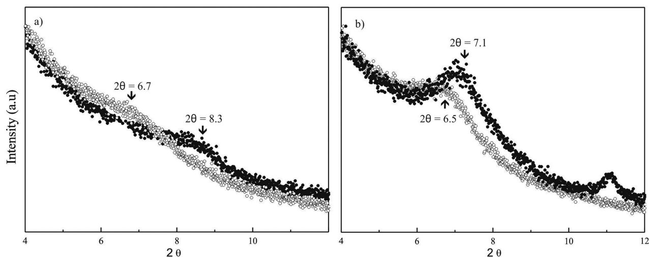
Figure 1. XRD patterns of (a) FeM and (b) NaM before (solid circles) and after (open circles) Atz adsorption.
