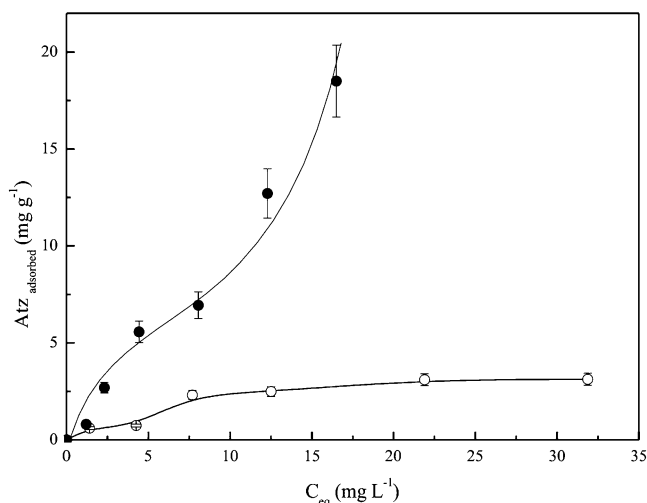
Figure 2. Effect of the interlaminar cation on the adsorption of Atz. Solid concentration, 1 g L -1 ; pH, 7.0, and NaNO 3 : 0.1 M. Solid circles, NaM; open circles, FeM. Lines are drawn only to serve as guides to the eyes.
