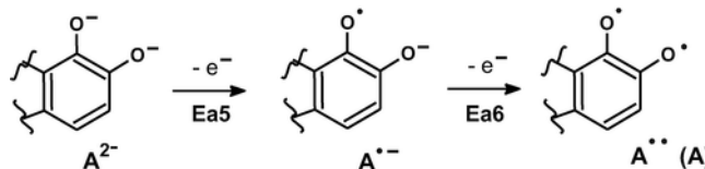
Scheme 8. Electro-oxidation reaction mechanism proposed for ALZ in solution of all studied solvents in presence of base.
