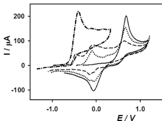
Fig. 5. Anodic CV of ALZ (5.04 mM) in DMF solution (—). Same solution with KOH added in different final concentrations: (•••••) 2.1 mM; (---) 5.2 mM; (-••••) 56 mM. v : 0.200 \text{ Vs}^{-1} ; supporting electrolyte: 0.10 M \text{NaClO}_4 . KOH was added from a solution of KOH in ethanol containing 0.051 g of anhydrous KOH per g of solution.
