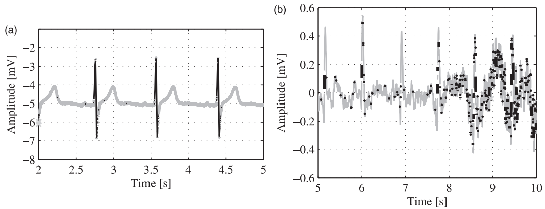
Figure 3. ECG sample signals. The original waveforms before compression are shown. Light grey traces correspond to segments that were encoded using 1 byte while black traces correspond to segments encoded using 2 bytes.
