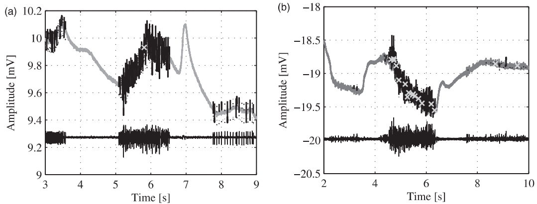
Figure 4. EMG sample signals. Upper traces are the raw waveforms while lower traces correspond to the same signal band-pass filtered in the usual EMG bandwidth of 10–450 Hz. The colour scheme is similar to Figure 3, with crosses representing samples coded with 3 bytes.
