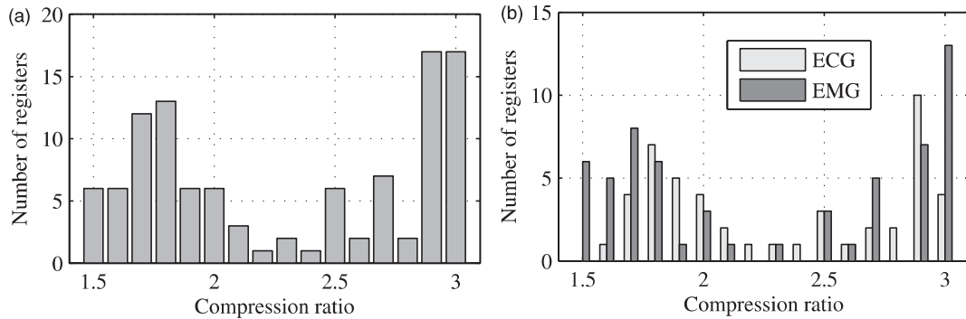
Figure 2. Compression ratios achieved for a database of ECG and EMG registers.
