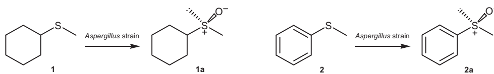
Fig. 1. Biotransformation of prochiral sulfides by Aspergillus strains.
