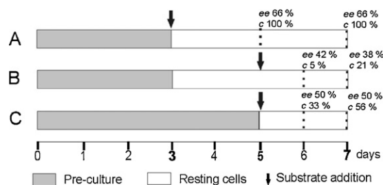
Fig. 2. Culture age and bio-reaction time using A. candidus resting cells. Arrows indicate the time when substrate 1 was added. Dotted lines show the day when samples were taken. c (%) and ee (%) determined by chiral GC analysis.
