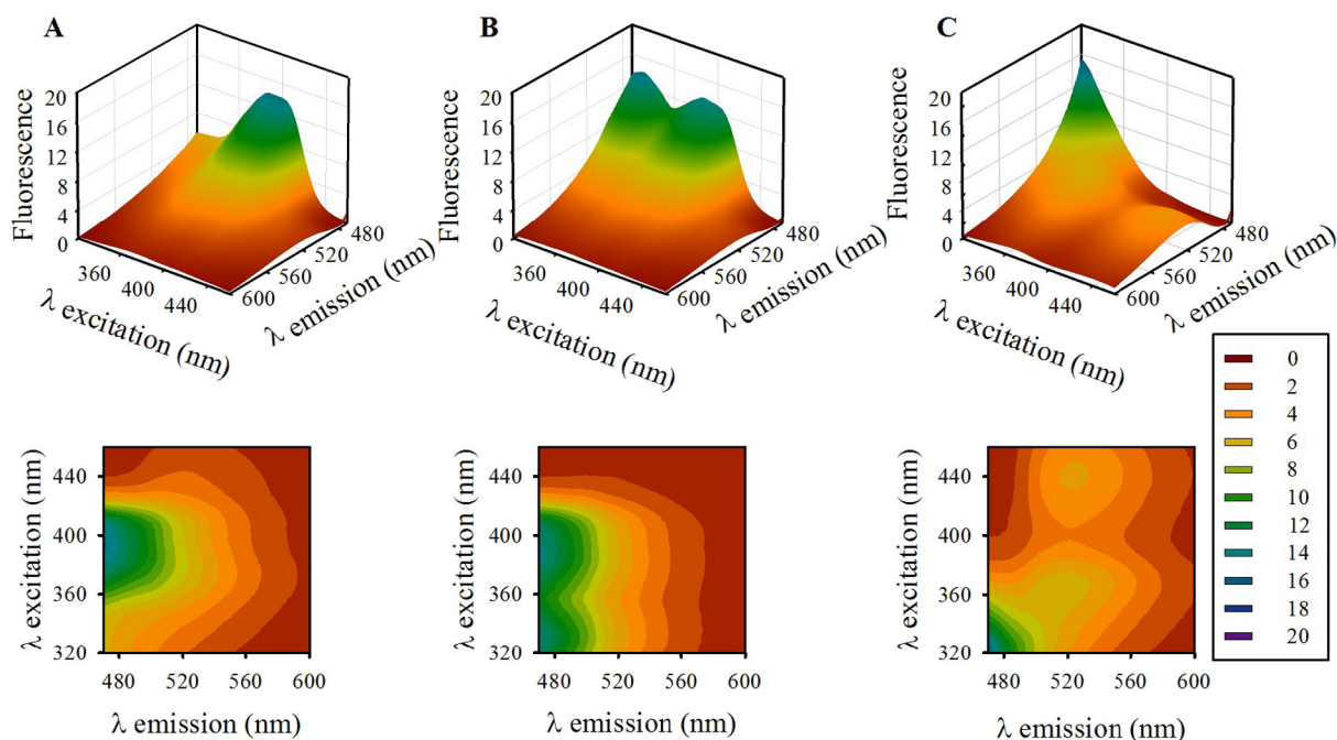
Fig. 3. Three-dimensional plots and the corresponding contour plots of excitation-emission fluorescence matrices for (A) a validation sample containing 0.10 \text{ mg L}^{-1} RF, (B) a test sample containing 0.08 \text{ mg L}^{-1} RF and 0.98 \text{ mg L}^{-1} OFL, and (C) a spiked human urine diluted (1:25) with 0.10 \text{ mg L}^{-1} RF.
