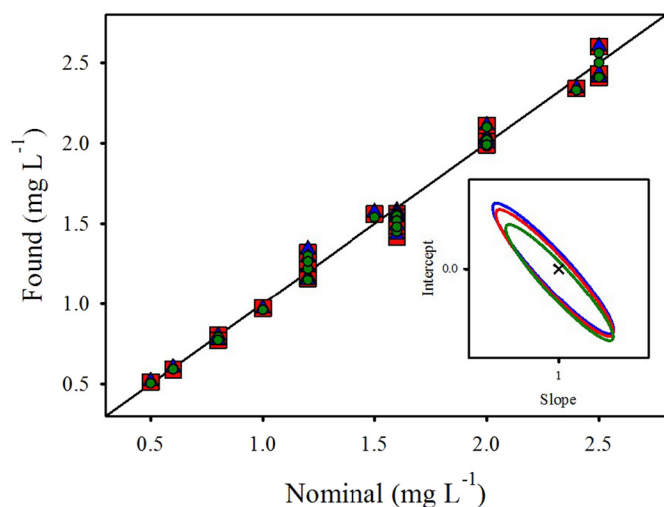
Fig. 6. Plots for RF predicted concentrations in spiked human urine samples as a function of the nominal values using PARAFAC in mode 2 (blue triangle up), U-PLS/RBL in mode 2 (red square) and N-PLS/RBL in mode 2 (green circle). The inset shows the corresponding elliptical joint regions (at 95% confidence level) for slope and intercept of the regression of PARAFAC in mode 2 (blue line), U-PLS/RBL in mode 2 (red line), and N-PLS/RBL in mode 2 (green line). The cross marks the theoretical (intercept = 0, slope = 1) point. (For interpretation of the references to color in this figure legend, the reader is referred to the web version of this article.)
