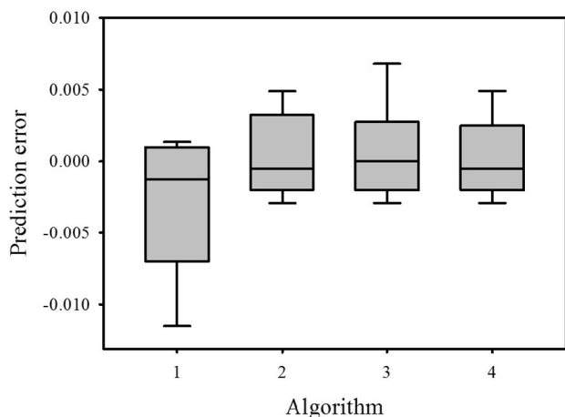
Fig. 4. Box and whisker plot of prediction results corresponding to the validation samples for RF. Algorithms are numbered in the horizontal axis as follows: (1) PARAFAC standard addition in mode 1, (2) PARAFAC standard addition in mode 2, (3) U-PLS/RBL standard addition in mode 2, and (4) N-PLS/RBL standard addition in mode 2. For each algorithm, the gray boxes are bounded by the 25% and 75% quartiles with the median inside, whereas the extreme levels correspond to 5% and 95% quartiles.
