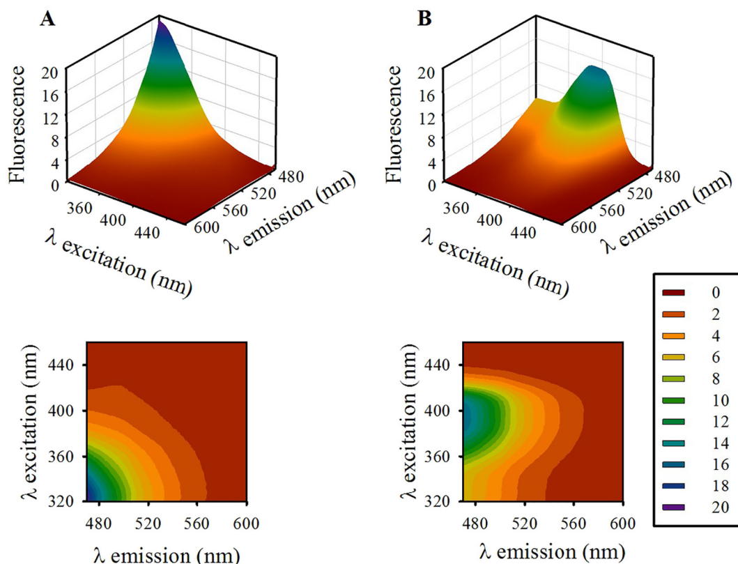
Fig. 2. Three-dimensional plots and the corresponding contour plots of excitation-emission fluorescence matrices for (A) a diluted (1:25) human urine and (B) diluted (1:125) blank urine.
