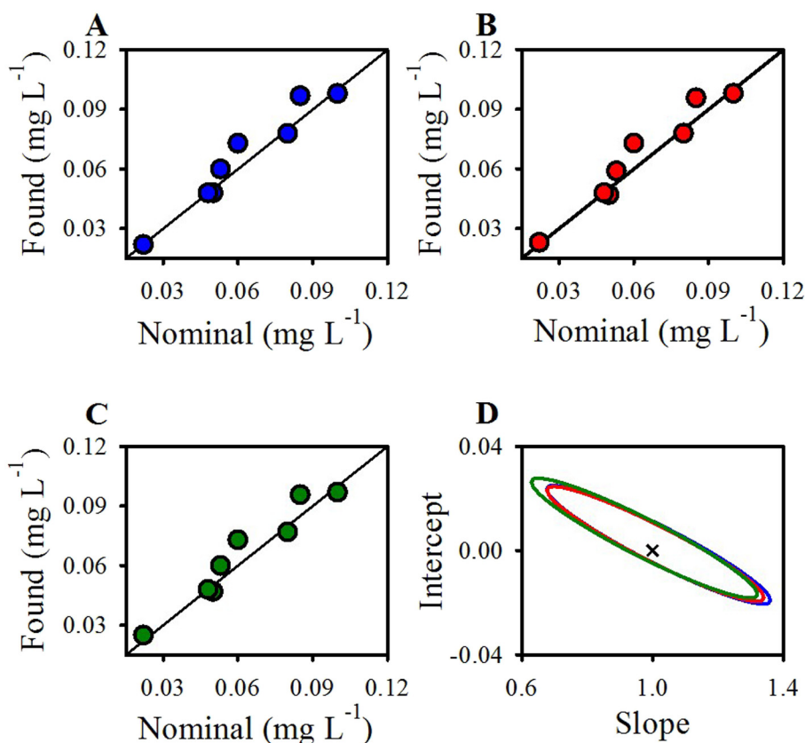
Fig. 5. Plots for RF predicted concentrations in test samples with interference as a function of the nominal values using (A) PARAFAC in mode 2, (B) U-PLS/RBL in mode 2, (C) N-PLS/RBL in mode 2 and (D) Elliptical joint regions (at 95% confidence level) for slope and intercept of the regression of PARAFAC in mode 2 (blue line), U-PLS/RBL in mode 2 (red line), and N-PLS/RBL in mode 2 (green line). The cross marks the theoretical (intercept = 0, slope = 1) point. (For interpretation of the references to color in this figure legend, the reader is referred to the web version of this article.)
