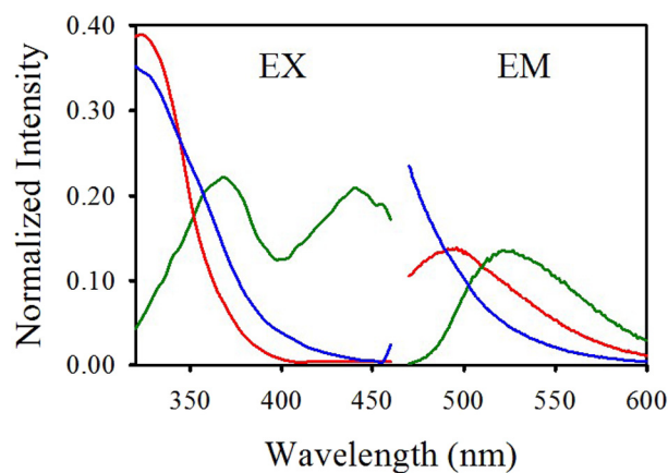
Fig. 1. Normalized excitation and emission fluorescence spectra of human urine diluted (1:25) (blue line), RF (green line) and OFL (red line). C_{RF} = 0.05 \text{ mg L}^{-1} , C_{OFL} = 0.25 \text{ mg L}^{-1} . (For interpretation of the references to color in this figure legend, the reader is referred to the web version of this article.)
