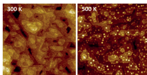
Figure 2. STM images for 0.1 ML Ni on CeO 2 (111) after deposition at 300 K and annealing to 500 K. The area covered by each image is 120 \text{ nm} \times 120 \text{ nm} .
