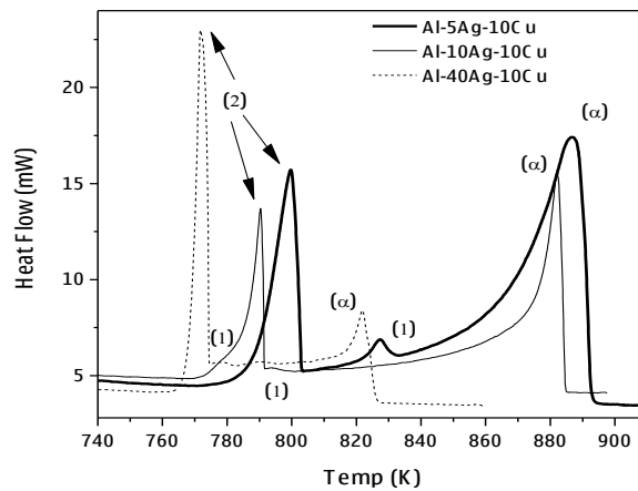
Fig. 5. Thermograms obtained by DSC for the AlAgCu non eutectic ternary alloys. In the curves is indicated the formation of the primary phase (α), binary (1) and ternary (2) eutectic.
