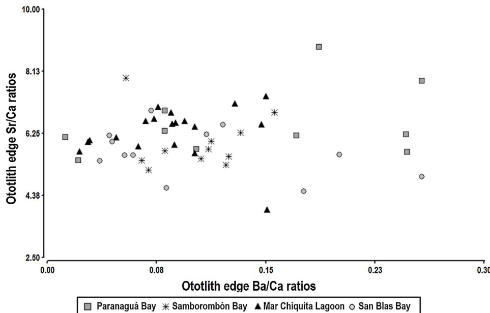
Fig. 6. Relationship between the otolith edge Sr/Ca and Ba/Ca ratios (mmol/mol) of Mugil liza for the sampling sites in the Southwestern Atlantic Ocean.
