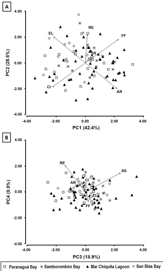
Fig. 3. Principal Component Analysis based on otolith morphometry data. A. Individuals projected along the first and second principal component axes; B. Individuals projected along the third and fourth principal component axes. Otolith indices: CI: circularity; RE: rectangularity; AR: aspect ratio; SS: percentage of the otolith area occupied by the sulcus; EL: ellipticity; and FF: form factor.
