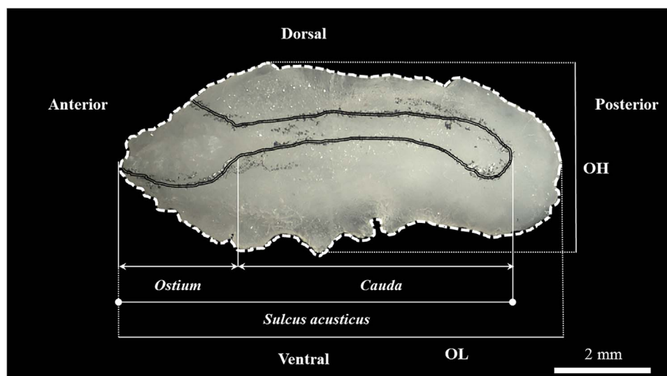
Fig. 2. Right sagitta otolith of Mugil liza . Features and measured variables: OL: otolith length; OH: otolith height; OP: otolith perimeter (dash white line); SP: sulcus perimeter (continuous black line).
