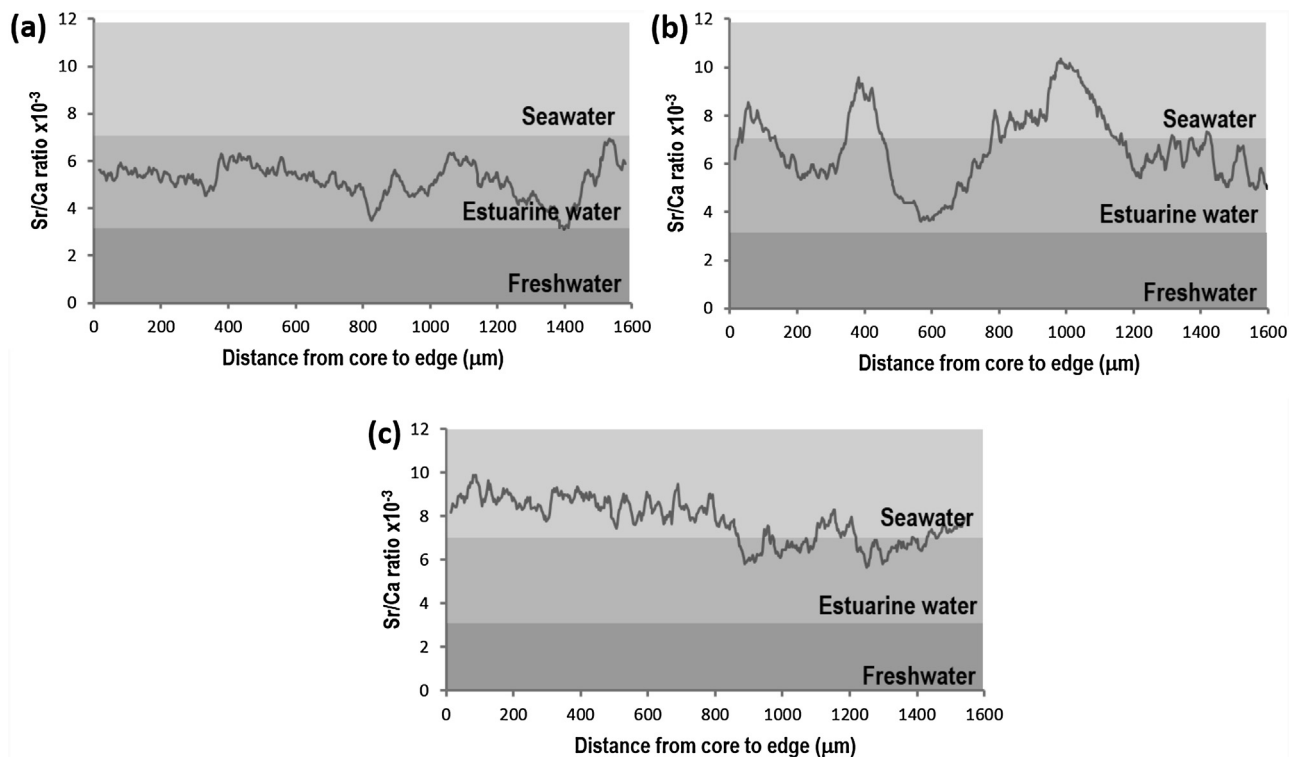
Fig. 4. Otolith life history profiles of Sr/Ca ratios for the 3 identified behavior patterns of Mugil liza in the four sampled areas in the Southwestern Atlantic measured by LA-ICP-MS from core to edge. Letters refer to identified groups: (a) Type I: estuarine resident (specimen from Mar Chiquita Coastal Lagoon, LS = 394 mm, female); (b) Type II: mixed (specimen from San Blas Bay, LS = 370 mm, female); and (c) Type III: seawater resident (specimen from Paranaguá Bay, LS = 370 mm, sex unknown).
