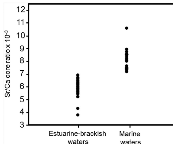
Fig. 7. Spawning grounds of Mugil liza sampled individuals related to Sr/Ca core ratio values. Microchemical thresholds considered were: estuarine-brackish waters, Sr/Ca: 3.5-7.0 \times 10^{-3} mmol/mol; and marine waters, Sr/Ca: > 7.0 \times 10^{-3} mmol/mol (Chang et al., 2004; Górski et al., 2015 and Wang et al., 2010).
