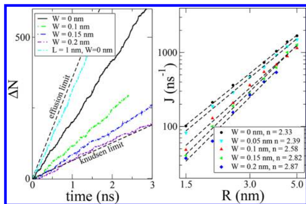
Figure 9. Left: Time evolution of \Delta N for nanotubes with different values of the atomic scale roughness W ( P_s = 9 atm and P_c = 1 atm). As W increases, diffusive reflections dominate and the Knudsen flow regime is approached. For low values of roughness and short nanotubes, the contribution of diffusive reflections is negligible and flow approaches the effusion limit. Right: Log–log plot of the flow J as a function of the nanotube radius for different values of W . Values of the n exponent fitted according to the power law J \propto R^n are indicated in the legends. Unless otherwise indicated, in these simulations, L was set to 30 nm.
