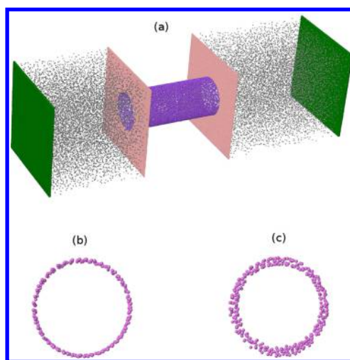
Figure 1. (a) View of the simulated system: Two reservoirs containing methane particles (gray) are joined by a cylindrical nanotube (violet), while independent pistons (green) perform pressure control in each reservoir. Pink particles constitute the reservoir walls. (b) Cross-sectional view of an atomically smooth nanotube ( W = 0 ). (c) Cross-sectional view of an atomically rough nanotube ( W = 0.1 \text{ nm} ).
