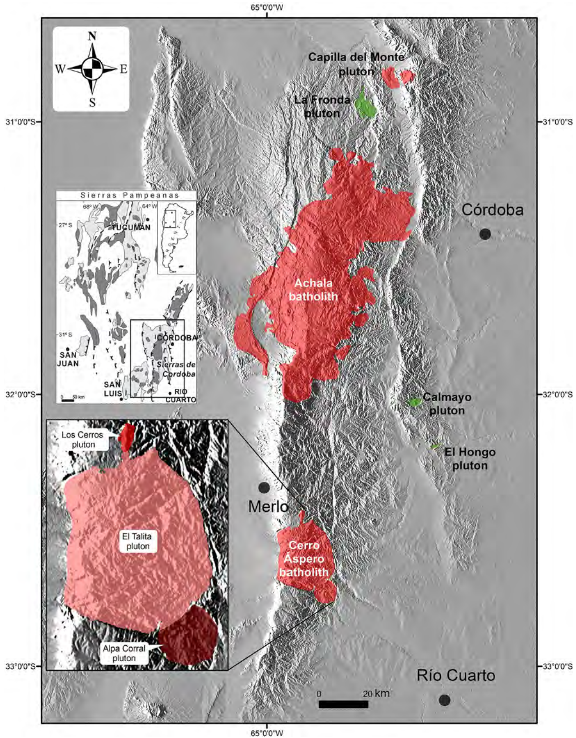
Fig. 1. Digital elevation model of the Sierras de Córdoba, showing location of the Cambrian-Ordovician small plutons (5–25 km 2 – shaded in green), and the large Achala (4000 km 2 ) and Cerro Aspero (440 km 2 ) batholiths, along with the Capilla del Monte pluton, belonging to Devonian magmatism (shaded in red). Inset at the top: Location of the Sierras de Córdoba (solid rectangle) in the context of the Sierras Pampeanas. Inset at the bottom: Location of the plutons comprising the Cerro Aspero batholith, from north to south: Los Cerros pluton, El Talita pluton and Alpa Corral pluton. (For interpretation of the references to colour in this figure legend, the reader is referred to the web version of this article.)
