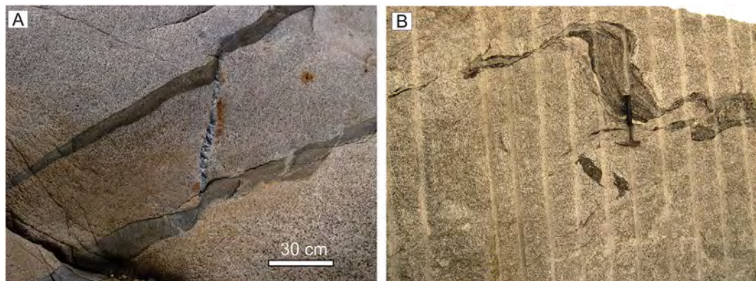
Fig. 8. (A) A pair of mafic dikes sheared in several locations. Note that shearing generally does not extend into adjacent trondhjemite, demonstrating its synmagmatic nature. In one locality, trondhjemite intrudes the shear zone (red arrow), in another quartz infills the shear zone that connects the two dikes. (B) Syn-magmatic shear bands folding, thinning and disaggregating a schlieren . (For interpretation of the references to colour in this figure legend, the reader is referred to the web version of this article.)
