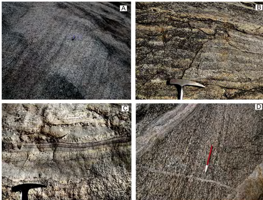
Fig. 4. Different types of layering. (A) Rhythmic isomodal layering defined by alternating bands of mostly quartz–feldspar composition (only minor biotite) and mafic bands with high biotite contents, homogeneously distributed throughout them. (B) Modally-graded layering marked by a sharp biotite-rich contact at the base and progressive decrease in biotite content towards the top contact. (C) Dike layering consisting of margin-parallel layered aplite and pegmatite bands. (D) Dike layering consisting of layers with varying amounts of biotite similar to layering in the host trondhjemite.
