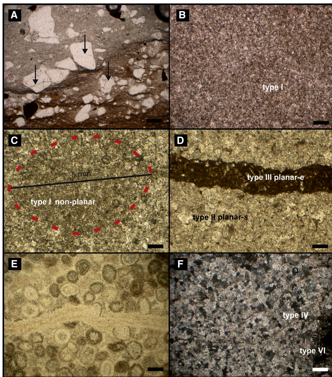
Fig. 6. Microphotographs from Villa Mónica Formation microfacies: (A) diamictite with dropstones = Fd; (B) dolomiticrite of type I; (C) type I (inner peloid); (D) type II, and III as the fill of veins; (E) type I and II in ooids; (F) type IV with a pore with type VI (scale bar: 200 \mu m).
