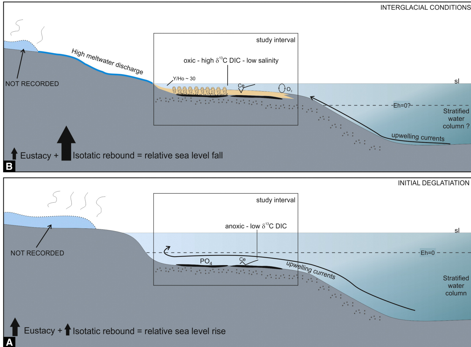
Fig. 11. Schematic representation to explain the trend in dissolved inorganic carbon (DIC) in \delta^{13}\text{C} , Ce anomalies related to redoxcline ( Eh = 0 ) and seawater salinity. (a) Paleoenvironment scheme of the lower Villa Mónica Formation with a stratified basin during initial deglaciation related to low Eh (positive Ce anomaly) and negative \delta^{13}\text{C} . (b) Paleoenvironment scheme of the upper Villa Mónica Formation with normal circulation of oxygen leading to negative Ce anomalies and positive \delta^{13}\text{C} , associated with high meltwater discharge during an interglacial interval.
