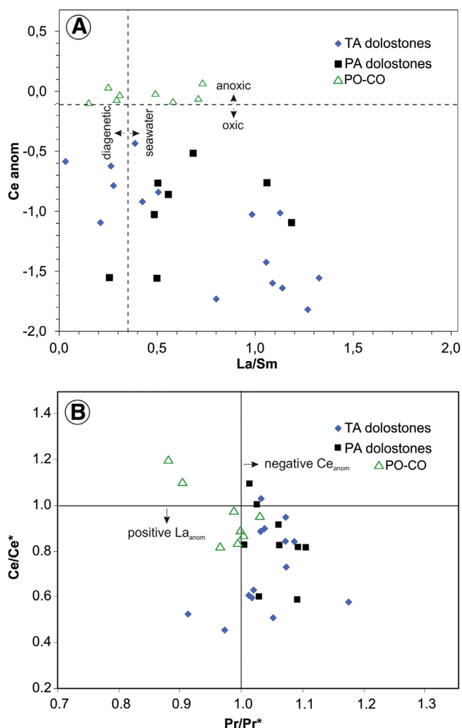
Fig. 7. A) Crossplot of Ce anomaly vs. La_N/Sm_N showing the distribution of dolomitized samples from Tres Antenas (TA) and Piedra Amarilla (PA) quarries. B) Ce/Ce^* vs. Pr/Pr^* diagram after Bau and Dulski (1996). This plot evaluates the possible overestimation of negative Ce anomalies due to La enrichment ( >1.0 = three samples) in dolostones of the Villa Mónica Formation.
