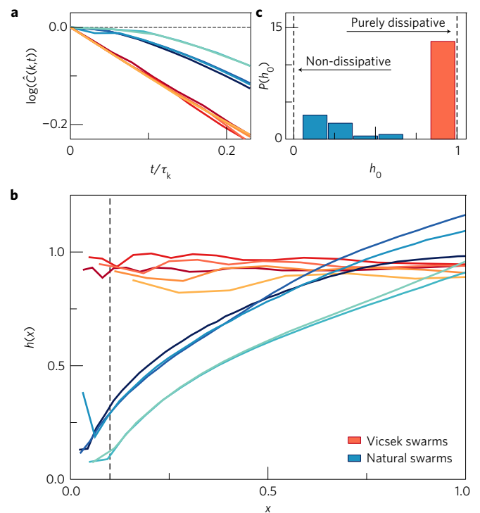
Figure 3 | Non-dissipative relaxation. a , The correlation in Vicsek swarms displays exponential relaxation (linear decay in semi-log scale), while natural swarms have a strongly non-exponential correlation function (flat derivative for small t ). b , To quantify the different form of the correlation we calculate the function h(x) defined in (7), where x = t/\tau_k ; in contrast with Vicsek, natural swarms are characterized by a small value of h(x) in the interval 0 < t < \tau_k . c , We compute the intercept h_0 = h(x=0.1) for all data and report its distribution: all natural swarms have a low first derivative, indicating the existence of non-dissipative modes, while Vicsek swarms have a purely dissipative peak at h_0 \sim 1 .
