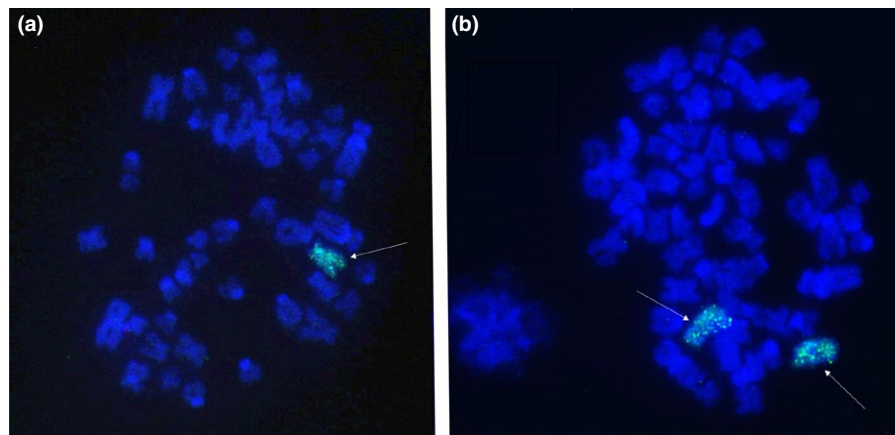
FIGURE 4 ZOO-FISH metaphases of Equus asinus (donkey) hybridized using Equus caballus (horse) probes. (a) 61,X metaphase. (b) 62,XX metaphase. Arrows show the EASX (X chromosome)
