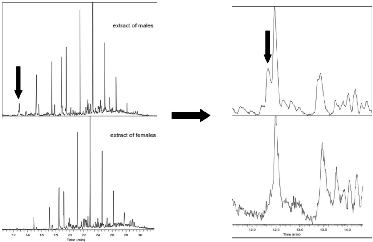
Fig. 1. Gas chromatogram of volatile extracts obtained from aeration of 20 males and females of Acrotomopus atropunctellus for 48 h, showing a male specific compound. Capillary column TR-5MS (30 m \times 0.25 mm \times 0.25 \mu m).
