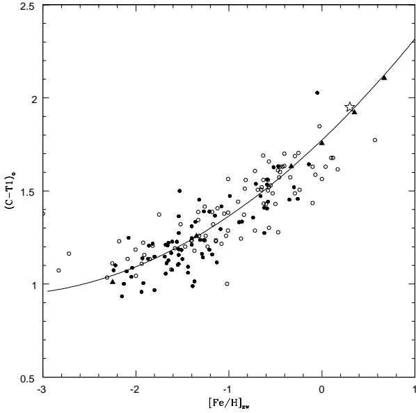
Figure 7. (C-T_1)_o colour versus metallicity [\text{Fe}/\text{H}]_{\text{sw}} on the Zinn and West scale relation derived from Milky Way clusters (filled dots) and globulars in NGC 3379, NGC 3923 and NGC 4649 (open dots). The star represents the nucleus of NGC 1399, triangles are models from Maraston (2004) (see text). The continuous line is a quadratic fit adopted as the mean calibration.
