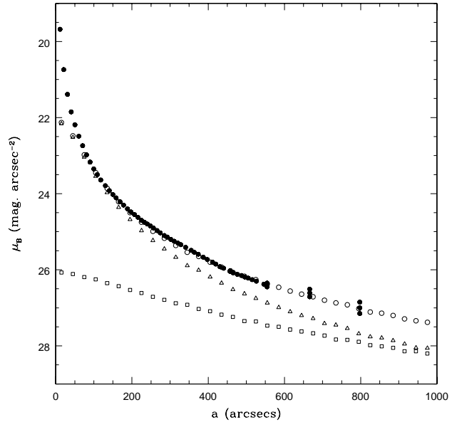
Figure 13. Observed B surface brightness profile for NGC 1399 (FFG05; filled dots) confronted with the model fit (open circles). This last profile was obtained from a bi-dimensional model image processed with the ELLIPSE task within IRAF. Squares and triangles represent the luminosity associated with the “blue” and “red” stellar populations. Note that the model fails inside 100 arcsec in galactocentric radius where the globular distributions shows a flat core.
