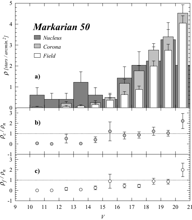
Figure 5. (a) Apparent LFs for the cluster nucleus, cluster corona and comparison field. (b) and (c) denote \rho_c/\rho_n and \rho_f/\rho_n as a function of V , respectively (see Section 3.1). Errors from Poisson statistics are also indicated.
