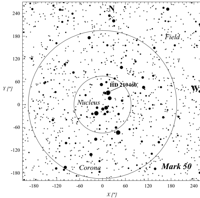
Figure 2. Finding chart of the area of Markarian 50 (V filter). The black solid circles, 1.25- and 3.25-arcmin radii, indicate the angular sizes found for the nucleus and the corona, respectively (see Section 3.1 and Fig. 4). For the coordinate reference system, the centre ( X = 0 ; Y = 0 ) corresponds to \alpha = 23^{\text{h}}15^{\text{m}}14^{\text{s}}.5 ; \delta = +60^{\circ}26'30''.0 . X - Y units are arcsec.
