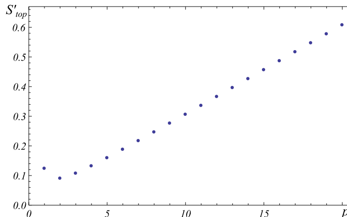
Figure 5. Dependence of the derivative of the topological entropy S'_{\text{top}}(p) with respect to p on the lens space L(p, 1) . For p \geq 2 , the dependence on p is monotonically increasing, and the asymptotic behavior for large values of p is linear.
