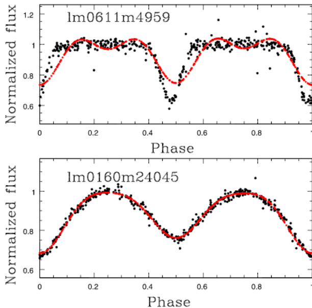
Figure 9. Examples of the Fourier fit obtained using six harmonics to model the light curve of detached (upper panel) and contact-like (bottom panel) binaries in our sample. Black dots represent the observational data, and red solid lines show the resultant Fourier fits. Six harmonics are clearly not sufficient to reproduce detached systems.
