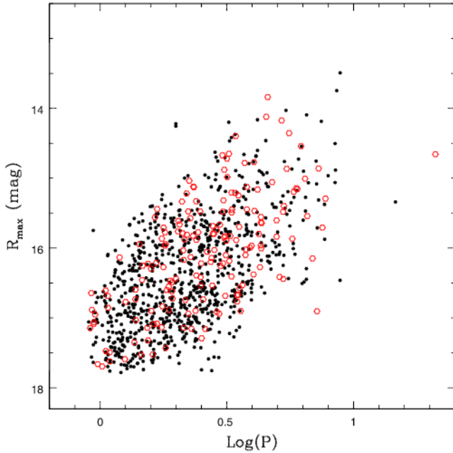
Figure 12. PL distribution in the R_{\text{EROS}} passband of 999 HEBs that have a counterpart in the VMC catalogue. Red open circles are objects we classified as contact binaries.
