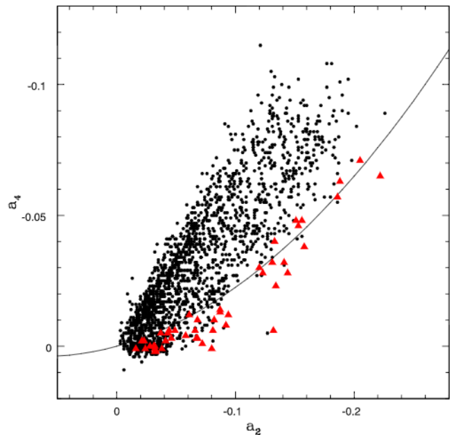
Figure 10. Fourier coefficients a_2 and a_4 of the 1768 HEBs in our sample. The solid curve is described by the relation a_4 = a_2(0.125 - a_2) which, according to Rucinski (1993), separates the regions of contact and non-contact binaries. Objects located below the line are considered to be contact systems. Red filled triangles identify objects classified as contact binaries in the OGLE III catalogue (see text for details).
