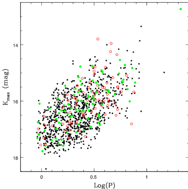
Figure 13. PL distribution in the K_s passband of 999 HEBs from our sample that have counterparts in the VMC catalogue. Red open circles are objects classified as contact binaries, and green filled circles are 90 contact EBs for which we have 13 or more epochs in the K_s light curves.
