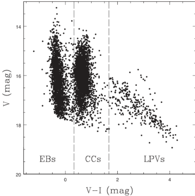
Figure 1. Colour–magnitude diagram of candidate CCs in the LMC, extracted from the EROS-2 catalogue on the basis of the period ( 0.89 < P_{\text{EROS}} < 15.85 d) versus luminosity ( 13.39 < B_{\text{EROS}} < 17.82 mag) diagram. The dashed lines correspond to (V - I) = 0.33 mag and (V - I) = 1.67 mag, respectively, and indicate the nature of the sources as classified in this study.
