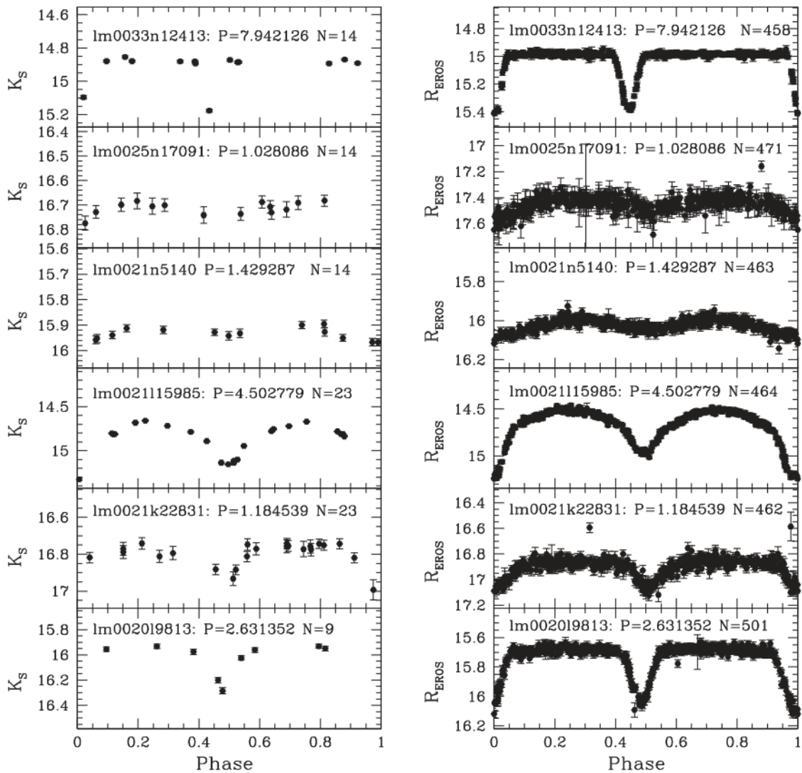
Figure 11. Light curves in the K_s (left panels) and R_{\text{EROS}} (right panels) passbands of example HEBs with a counterpart in the VMC catalogue. P – period (d), N – number of observations in the corresponding passband.
