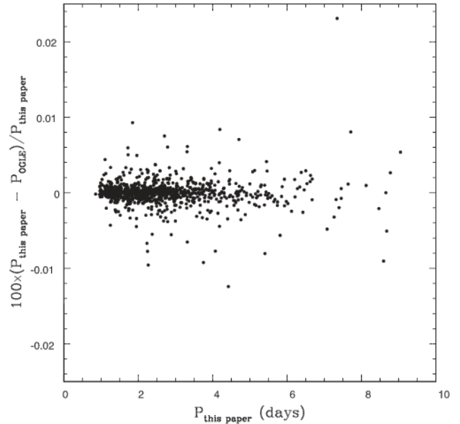
Figure 7. Comparison between periods adopted in this paper and those in the OGLE III and OGLE IV catalogues for the 1072 EBs in common. Two objects, namely lm0185123772 and lm0030n12500, were not included because their OGLE periods differ significantly from our values (see text and Fig. 8 for details).
