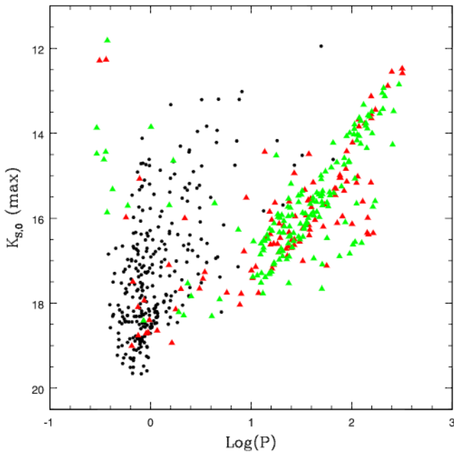
Figure 16. PL distribution at K_{s,0} maximum of the 563 contact binaries shown in Fig. 14. Black dots are objects with (V - I) < 0.3 mag, and red triangles are objects with (V - I) \geq 0.3 mag of which those with 13 or more epochs in the K_s band are marked in green.
