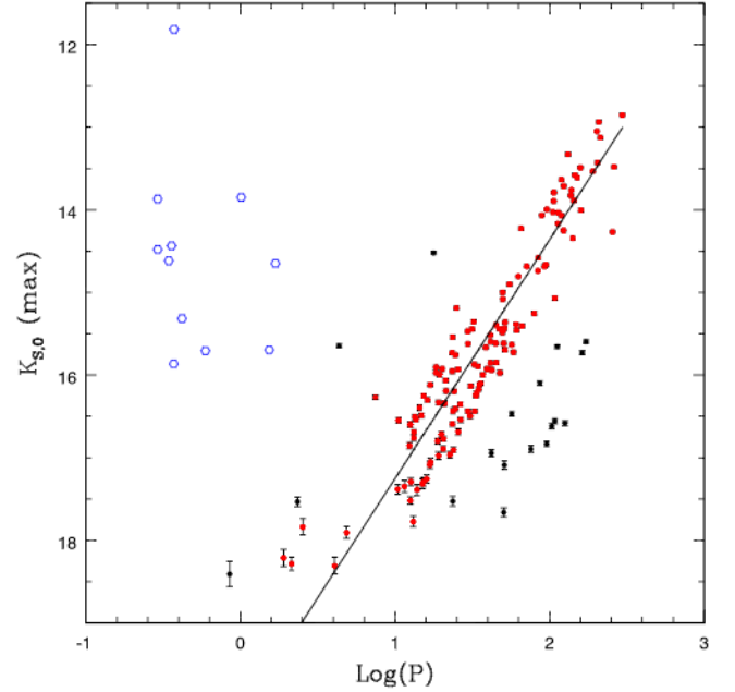
Figure 17. PL distribution of contact binaries containing red giant components. Blue open circles are candidate HEBs falling in the region of binaries with red giant components (their errors are smaller than the size of the circles), red and black dots represent EBs which deviate less (red) and more (black) than 3\sigma from a linear regression, respectively. The line is the weighted linear fit obtained from the objects marked in red.
