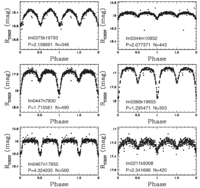
Figure 2. Examples of the R_{\text{EROS}} light curves for LMC EBs detected in the EROS-2 candidate CCs data set. P – period (d), N – number of observations.
