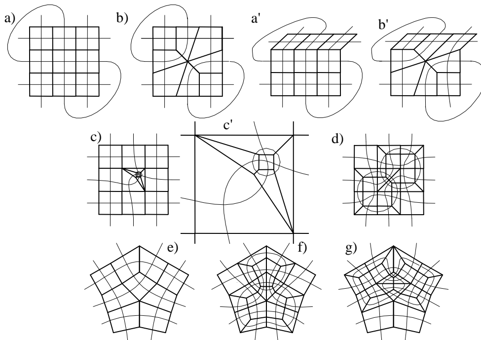
Figure 10: Effect of splitting on the mesh and some ways for removing an element
