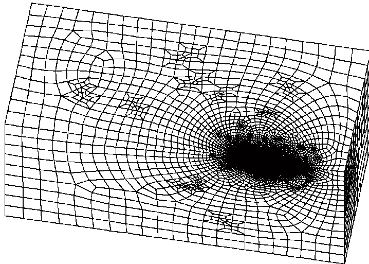
Figure 13: Effect of removing self-intersections in a mesh for the water around a sailboat (detail and complete mesh).
