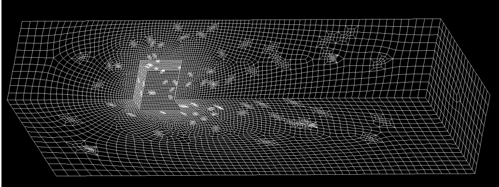
Figure 12: Mesh for a rectangular channel with a cubic obstruction.
