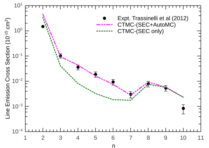
FIG. 7. (Color online) CTMC line emission cross sections for the 1snp \rightarrow 1s^2 transitions following 7 keV/amu \text{Ar}^{17+} + \text{Ar} charge-exchange collisions. The experimental data are those of Trassinelli et al. [27].
