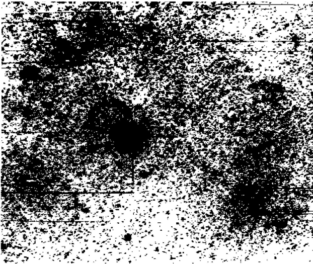
Figure 1. H\alpha image in (\alpha, \delta) coordinates showing the two concentric rings around WR 85 (taken from Marston et al. 1994). North is up and East is to the left.
