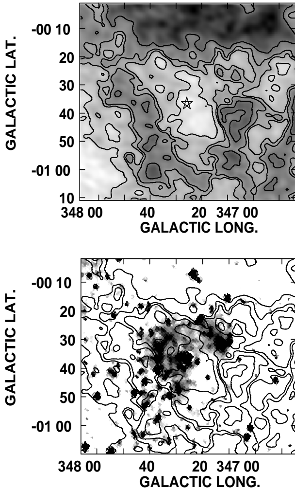
Figure 3. Top panel: HI column density distribution surrounding WR 85 within the velocity interval -28.0 to -16.5 km s ^{-1} . The grayscale corresponds to (1.2-1.7)\times 10^{21} cm ^{-2} and the contour lines are 1.2 , 1.4 , 1.5 and 1.6\times 10^{21} cm ^{-2} . The star symbol indicates the position of the WR star. Bottom panel: Overlay of the SHASSA H \alpha image of the nebula and the same HI contours of the top panel. H \alpha units are arbitrary.
