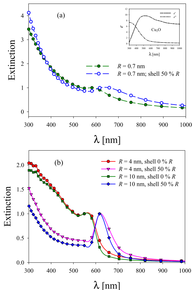
FIG. 1. Theoretical optical extinction spectra of copper bare core Nps compared with a core-shell \text{Cu-Cu}_2\text{O} Nps with the same core and 50% of shell thickness: (a) subnanometric and (b) nanometric. The shell produces a measurable redshift of the plasmon peak. Inset in panel (a) shows the dielectric function of \text{Cu}_2\text{O} taken from Palik.
