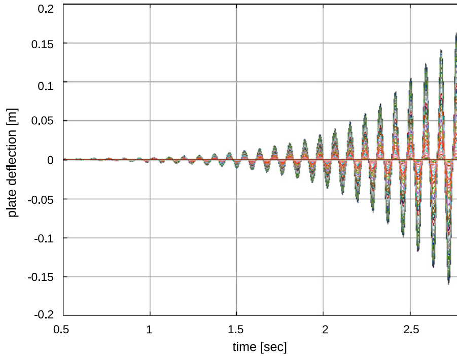
Fig. 18. Strong partitioned scheme in a coarse mesh.
