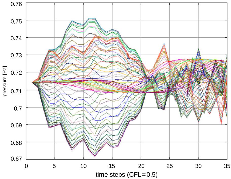
Fig. 16. Unstable weak coupling for m = 0.0135 and CFL = 0.5 .
