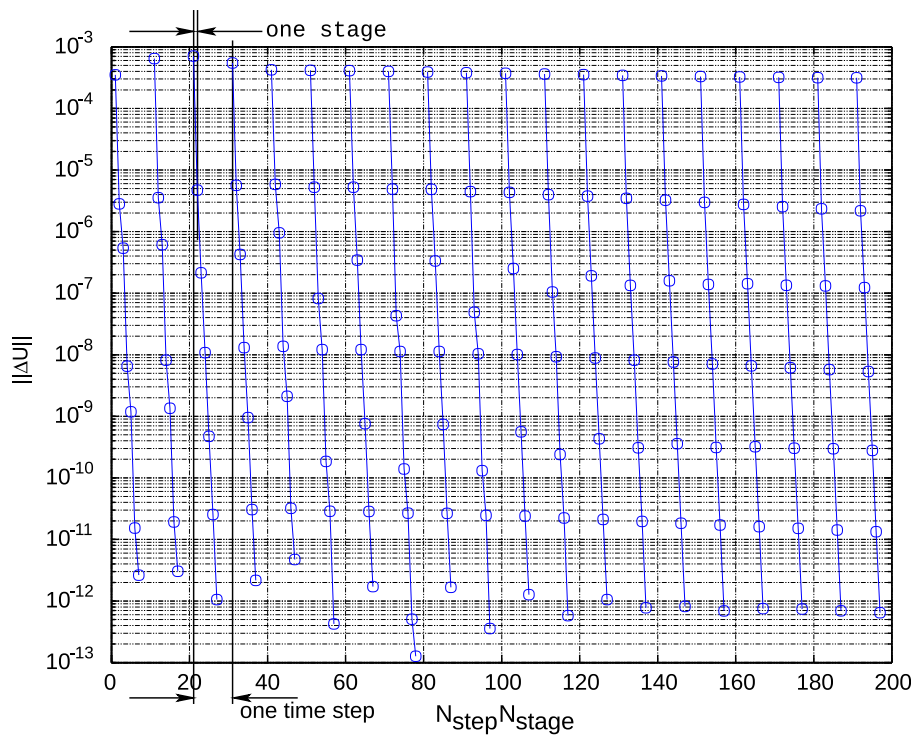
Fig. 13. Convergence of structure state in stage loop.
