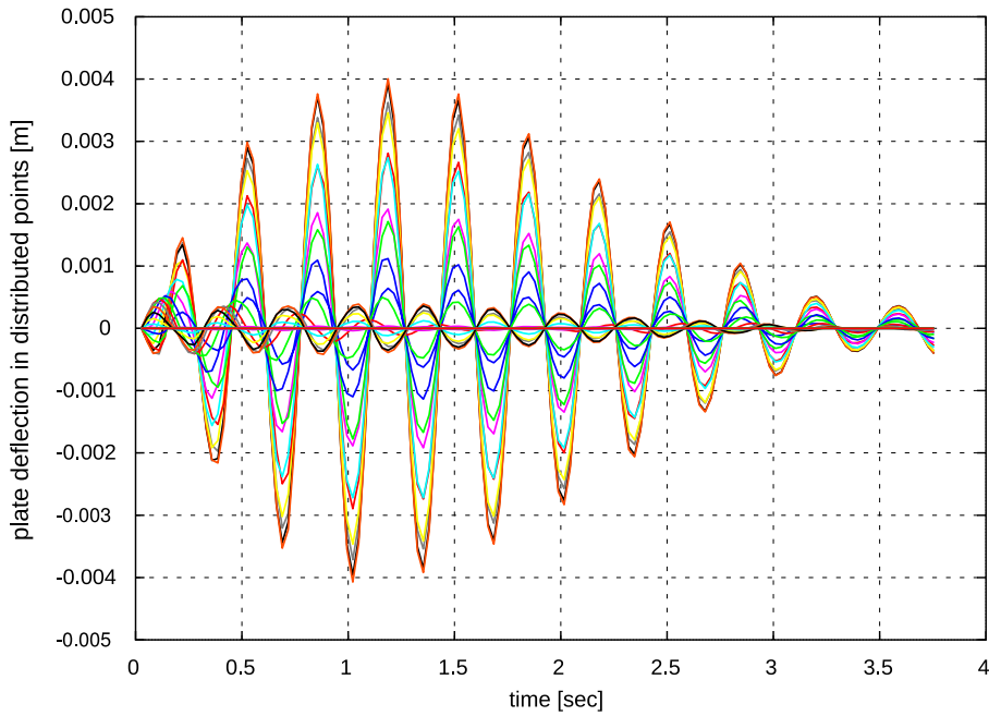
Fig. 4. Plate deflection in distributed points along plate at M = 2.225 .
