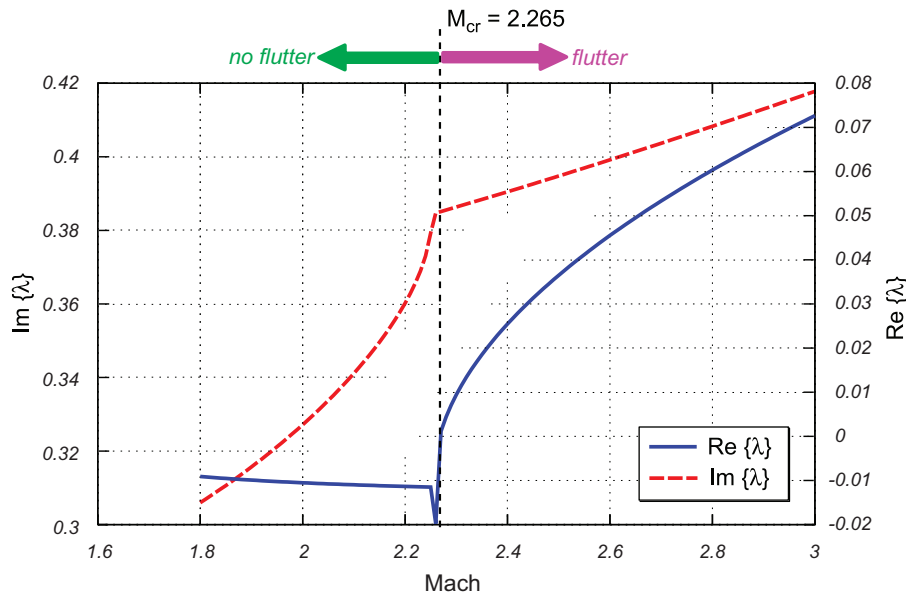
Fig. 2. Lowest frequency mode for test case.
