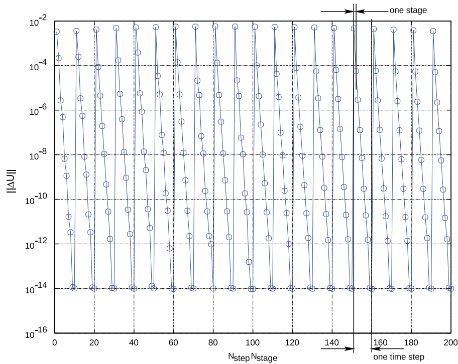
Fig. 12. Convergence of fluid state in stage loop.
