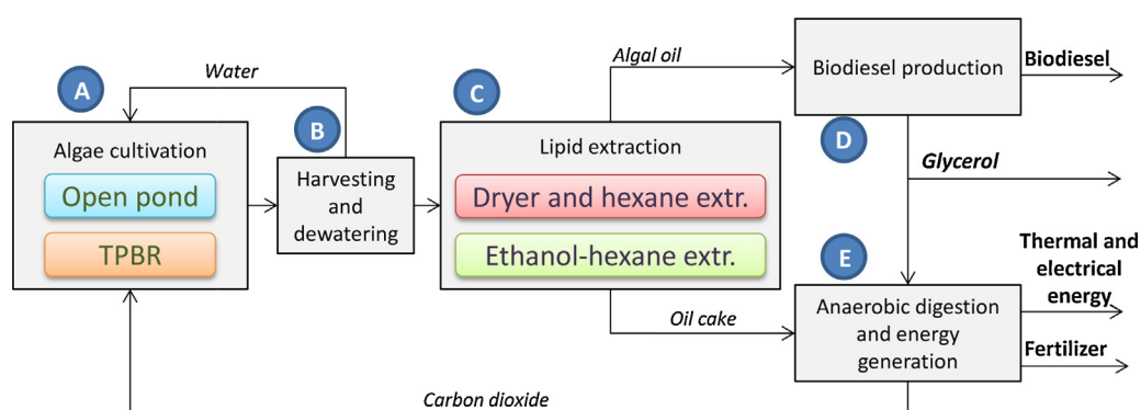
Fig. 2 – Simplified process flow diagram for the proposed integrated biorefinery.
