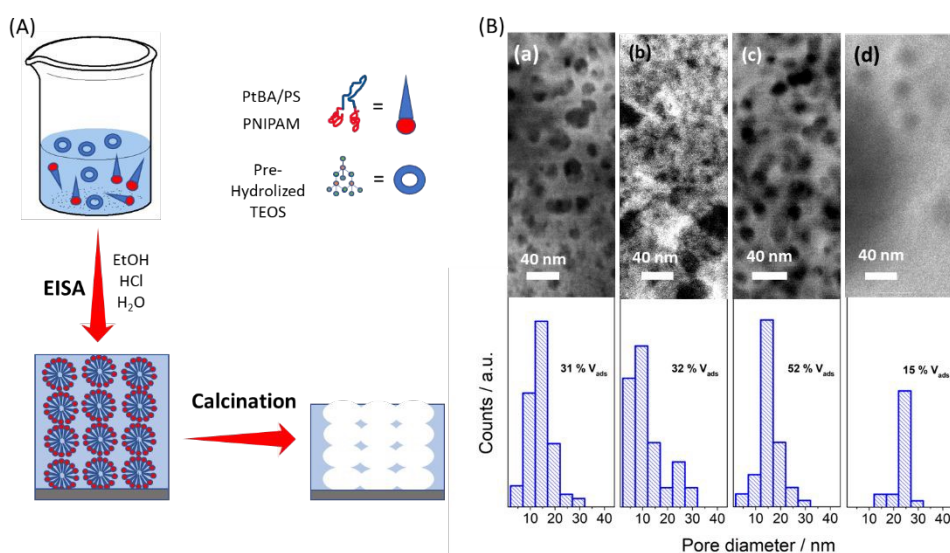
Figure 2. A) On the left scheme of the synthesis of the MTF. B) Histogram showing pore distribution based on SEM images for MTF based on the synthesized templates: PN-PB-24 (a), PN-PB-48 (b), PN-PS-12 (c), PN-PS-24 (d). The surface was homogenous though the whole sample, pore count ranges from 25 to 110 depending on the pore density. Pore volume was calculated through ellipsometry measurements at 0 and 100 % humidity.
