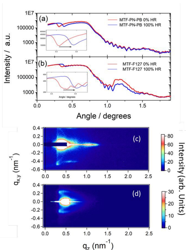
Figure 4. X-ray Reflectometry results obtained at low and high RH for (a) MTF-PN-PB-24 and (b) MTF-F127. Insets: critical angle displacement upon water adsorption. GI-SAXS patterns for (c) MTF-F127 and (d) MTF-PN-PB24.
