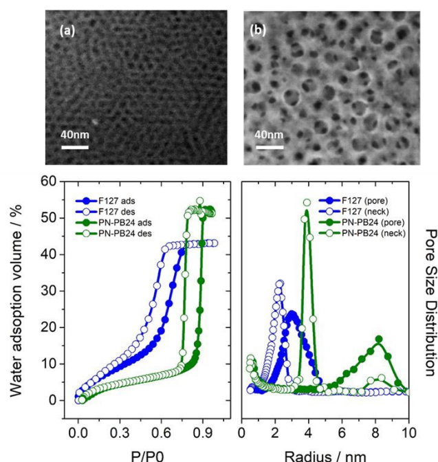
Figure 3. SEM analysis of the films surface for MTF-F127 (a) and MTF-PB-PB-24 (b) samples. EEP isotherm (b) and pore distribution analysis (c) for MTF-PN-PB-24 (green) and MTF-F127 (blue)
