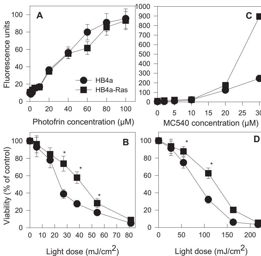
Fig. 1. PII and MC540 intracellular accumulation and response to PDT of HB4a and HB4a-Ras cells. Intracellular accumulation of PII (A) or MC540 (C) after 2 h exposure of cells to different PS concentrations. Survival after PDT mediated by PII or MC540 after 2 h exposure to 10 µM PII (B) or 20 µM MC540 (D) and different light doses was shown. Data represent the mean \pm SD for three independent experiments performed in duplicates. * p < 0.05 between HB4a- and HB4a-Ras (ANOVA followed by Tukey's test).
