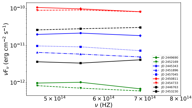
Figure 6. Examples of AO 0235+164 optical intraday SEDs during three different states of brightness: (i) the green lines represent SEDs during quiescent states ( \nu F_\nu (erg cm -2 s -1 ) < 10 -12 ), (ii) the blue lines show SEDs during moderately bright states (10 -12 < \nu F_\nu (erg cm -2 s -1 ) < 3 × 10 -11 ), and (iii) the red lines show SEDs during outbursts ( \nu F_\nu (erg cm -2 s -1 ) > 5 × 10 -11 ). The black lines are examples of SEDs with spectral hardening on JD 2,446,763 and JD 2,453,230.
