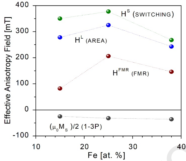
Figure 7. Different effective anisotropy field values in the arrays, determined by the three methods —by applying the area method to evaluate quasistatic hysteresis in the major hysteresis loops; through FMR measurements; and the effective anisotropy field acting during the magnetization switching mechanism responsible for coercivity. Field values calculated using Eq. (2), considering only magnetostatic interactions in porous systems are also shown.
