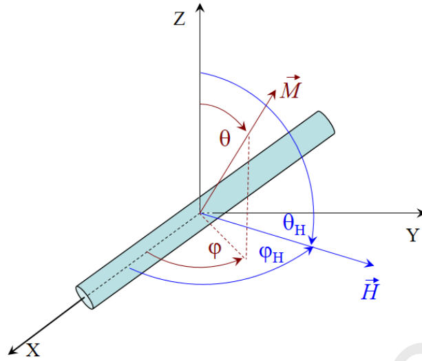
Figure 4. Schematic representation of a single nanowire and the convention used for polar and azimuthal angles of \vec{M} ( \theta , \varphi ) and \vec{H} ( \theta_H = \pi/2 , \varphi_H ).
