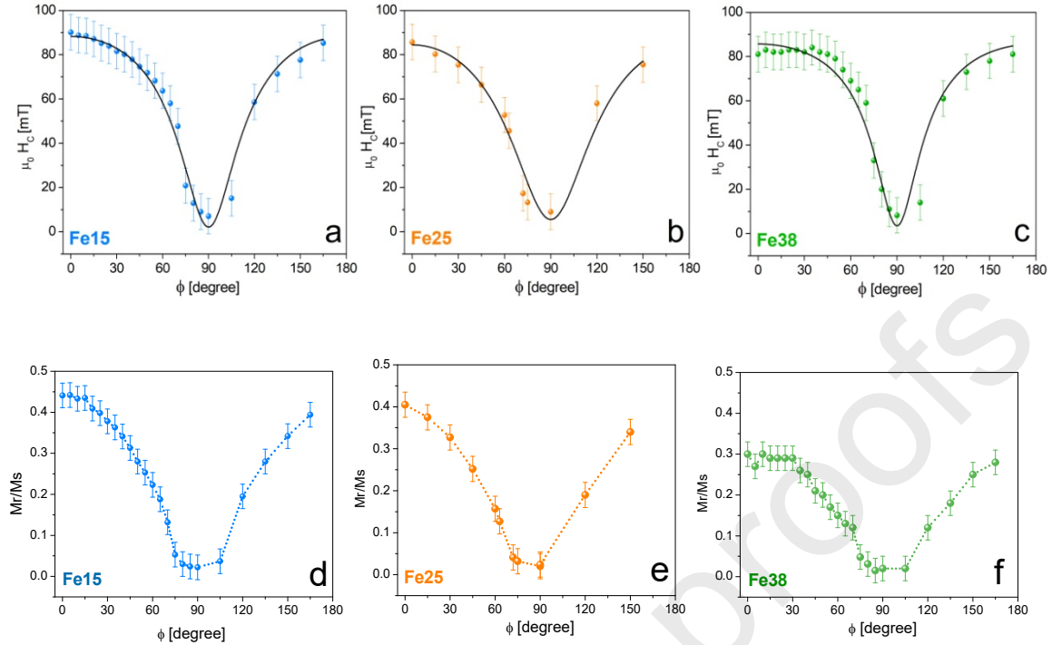
Figure 6. Angular dependence of the coercive field \mu_0 H_C and the relative remanence M_R/M_S for the NW arrays investigated: (a, d) Fe15; (b, e) Fe25; (c, f) Fe38. The solid lines in \mu_0 H_C plots correspond to fits of Eq. (9) to the experimental data. Dotted lines in M_R/M_S curves are displayed as a guide to the eye.
