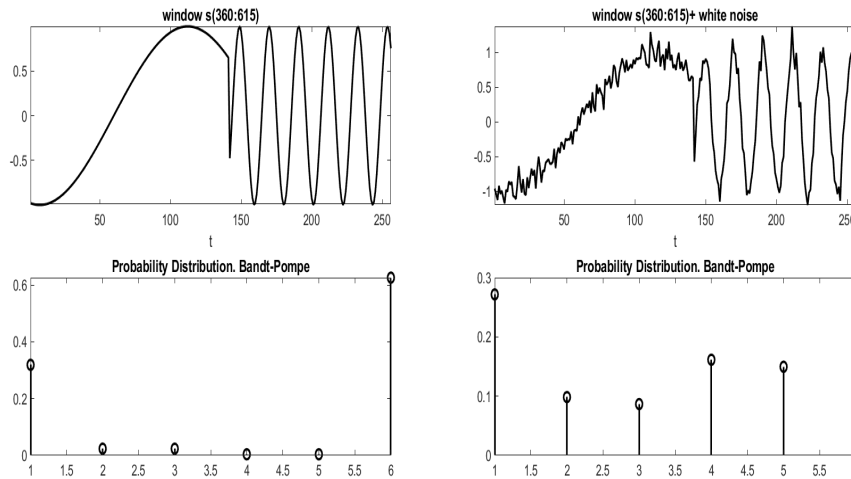
Figure 5: Permutation entropy of the window S_I(p) = 0.49 (left). Permutation entropy of the window adding white noise S_I(p) = 0.96 (right).
