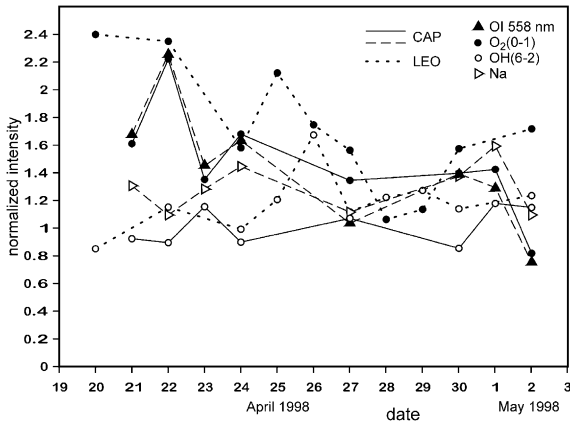
Fig. 2. Nocturnal mean airglow intensities at LEO (dotted lines) and CAP (solid and dashed lines), 20 April–2 May 1998. The emissions shown are OH(6–2) (open circles), Na (open triangles), O 2 (0–1) (solid circles), and OI 558 nm (solid triangles). Intensity units are relative to long-term (several-year) means.
