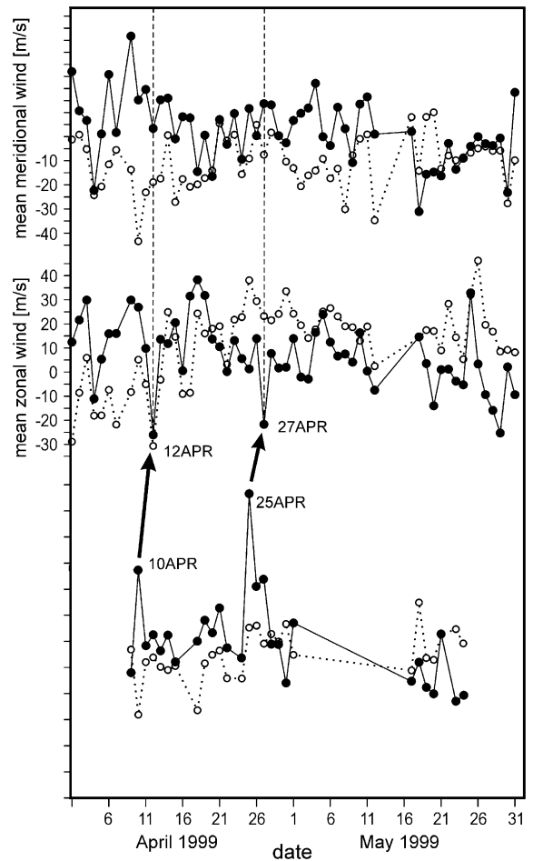
Fig. 3. Nocturnal mean airglow intensities at El Leoncito in April and May 1999 compared to daily means of meridional and zonal meteor wind components at Cachoeira Paulista. Solid dots and lines correspond to the upper level emission (O 2 , at 95 km nominal), and mean radar winds averaged over 91–98 km; open circles and dotted lines are for the lower altitude emission (OH, at 87 km), and radar winds at 82–88 km.
