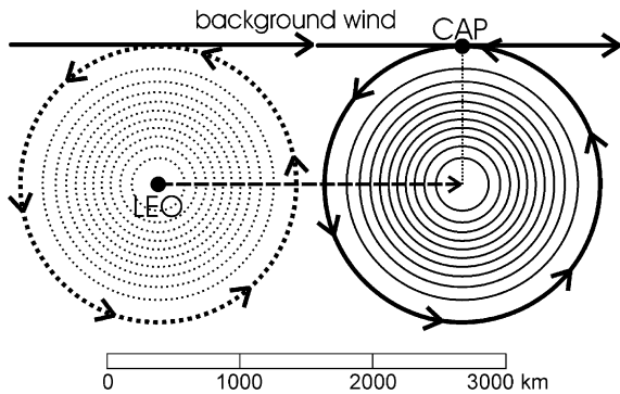
Fig. 6. Hypothetical mesopause region temperature and wind field in a plane map view over El Leoncito (LEO, 31.8°S 69.2°W) and Cachoeira Paulista (CAP, 22.7°S 45.0°W). Concentric circles show isotherms (with higher temperature towards the center), circles with arrows show the corresponding thermal wind. The pattern (dotted) centered over LEO corresponds to the time of the airglow burst observed there, and the other one (solid) to the maximum wind disturbance at CAP, about two days later.
