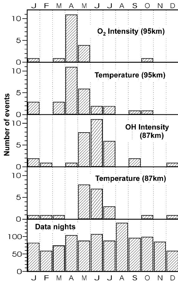
Fig. 1. Monthly distribution of high nocturnal means (based on observations at El Leoncito, 5 August 1997–25 September 2002), with respect to the four different parameters. The monthly coverage of observations is shown in the lowest panel.
