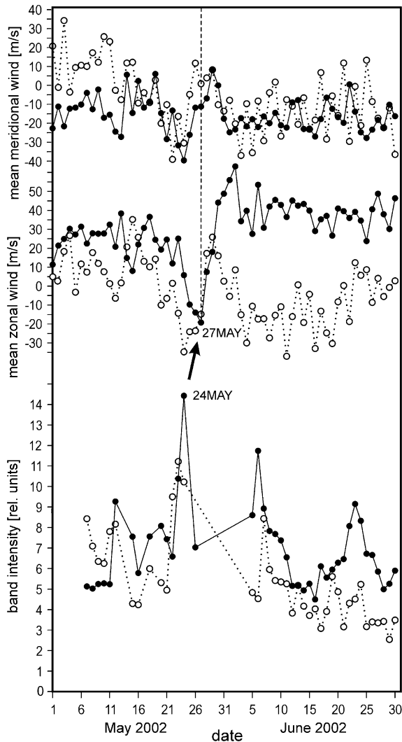
Fig. 5. As Figs. 3 and 4, but for May and June 2002. Same symbols as Fig. 4 (solid dots and lines: OH emission at 87 km, and radar winds at 82–88 km; open circles and dotted lines: O 2 emission at 95 km, and radar winds at 91–98 km).
