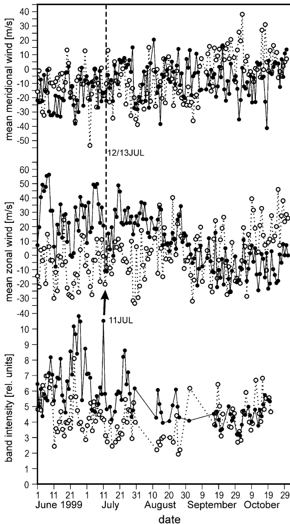
Fig. 4. As Fig. 3, but for June–October 1999. Notation is opposite to the one in Fig. 3; solid dots and lines: OH emission at 87 km, and radar winds at 82–88 km; open circles and dotted lines: O 2 emission at 95 km, and radar winds at 91–98 km.
