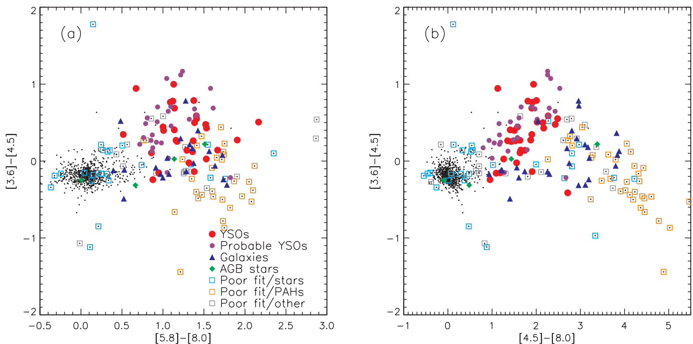
FIG. 2.— (a) IRAC [3.6] - [4.5] vs. [5.8] - [8.0] color-color diagram of N66. The black dots represent all detected sources (primarily stars); the red circles represent objects that can only be fit by YSO models; the smaller purple circles represent objects that are best fit by YSO models, although galaxy and/or AGB fits with significantly higher \chi^2 values are also acceptable; the blue triangles are background galaxies; and the green diamonds are AGB stars. The squares represent sources for which satisfactory fits were not obtained: the cyan symbols have SEDs that suggest they are likely to be stars, the orange symbols are sources that are contaminated by PAH emission features, and the gray symbols are the remaining unclassified poor fits. Note that the separation of YSOs from the other classes of sources is not very clean in this diagram. (b) IRAC [3.6] - [4.5] vs. [4.5] - [8.0] color-color diagram of N66. Symbols are the same as in (a). This plot offers the best separation of YSOs from the various contaminants, although there are still a few extragalactic sources that have colors similar to the YSOs.
