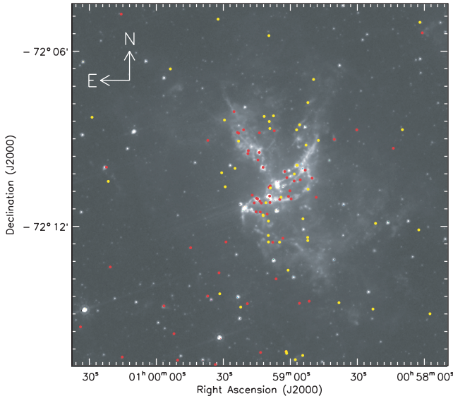
FIG. 3.— Spatial distribution of YSOs in N66, overplotted on an image of the 8.0 \mu\text{m} emission. The red circles represent objects with SEDs that can only be fit by YSO models, and the yellow circles represent objects that are probably YSOs but can be fit by other source types as well (albeit with significantly higher \chi^2 values). The image is displayed on a logarithmic scale from 4 to 20 \text{ MJy sr}^{-1} .
