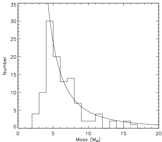
FIG. 5.—Mass function of YSOs in N66. The solid curve shows the best-fitting Salpeter IMF, which provides a reasonable fit to the data above 4 M_\odot , where the observational incompleteness becomes severe.
