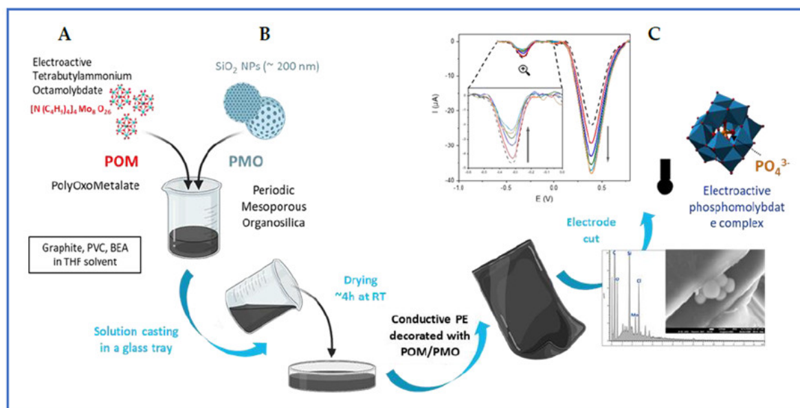
Figure 4. Scheme for the E-sensor preparation for phosphate detection in the two formulations adopted (A,B) and signal of enhanced sensitivity measured in presence of DIP (C).
