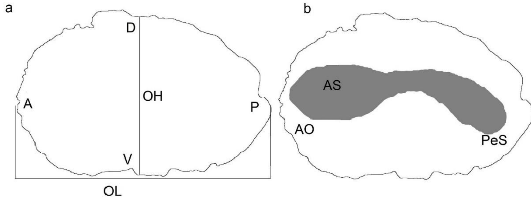
Figure 2. Scheme of linear morphometry applied to the right otolith of Opsanus beta collected in the Subtropical Southwestern Atlantic Ocean. a) A: anterior region, D: dorsal region, V: ventral region, P: posterior region, OL: maximum longitudinal length, OH: maximum perpendicular height. b) AO: area of the otolith and AS: area of the sulcus acusticus and PeS: perimeter of the sulcus acusticus .
