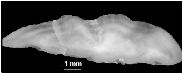
Figure 3. Cross-section of an Opsanus beta otolith ( sagitta ) female specimen TL = 25 cm, collected in the Paranaguá Estuarine Complex in the Subtropical Southwestern Atlantic Ocean.
