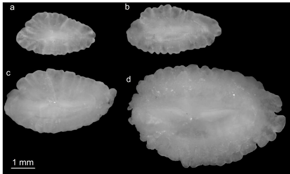
Figure 5. Photograph of the inner face of the right sagitta otolith of Opsanus beta throughout its ontogenetic development: a) 8.7 cm interval 5-10 cm, b) 10.5 cm interval 10.1-15 cm, c) 17.8 cm interval 15.1-20 cm, and d) 23.7 cm interval 20.1-25.
