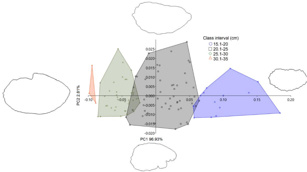
Figure 7. Scatterplot of the principal component analysis of the shape indices of the sagitta otolith of Opsanus beta along its ontogeny Subtropical Southwestern Atlantic.
