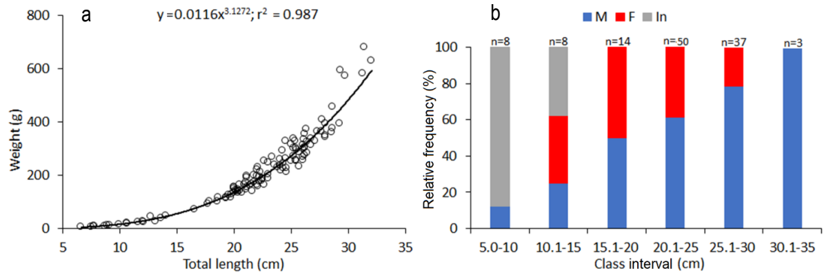
Figure 4. a) Length-weight relationships, b) distribution of sexual frequency per class interval of Opsanus beta in the Subtropical Southwestern Atlantic. M: males, F: females, Im: immatures.
