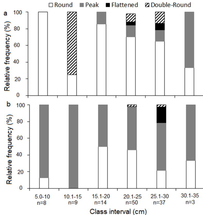
Figure 6. a) Frequency distribution of types anterior otolith regions, b) frequency distribution of types posterior otolith regions by interval class Opsanus beta Subtropical Southwestern Atlantic Ocean.
