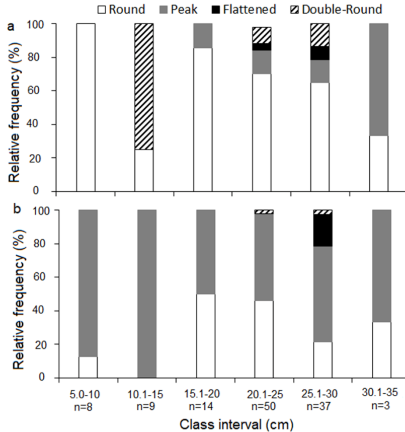
Figure 8. a) Frequency distribution of types anterior otolith regions, b) frequency distribution of types posterior otolith regions by interval class Opsanus beta Subtropical Southwestern Atlantic Ocean.
