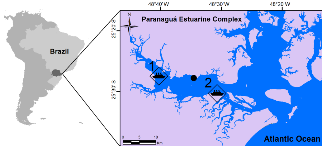
Figure 1. Sampling sites of Opsanus beta in the Paranaguá Estuarine Complex in the Subtropical Southwestern Atlantic Ocean. The black circle is the site of the sample, and the ship is the position of the Antonina (1) and Paranaguá Port (2).
