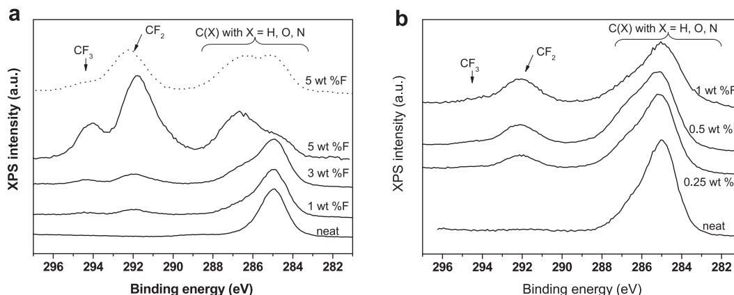
Fig. 5. High-resolved C_{1s} spectra of films of neat system, and fluorinated epoxy networks: a) FES3-DGEBA-JEFFAMINE (dashed line) containing 5 wt % F, and FED3-DGEBA-JEFFAMINE (solid lines) containing 1, 3 and 5 wt % F; and b) FES3-DGEBA-MCDEA containing 0.25, 0.5 and 1 wt % F.
