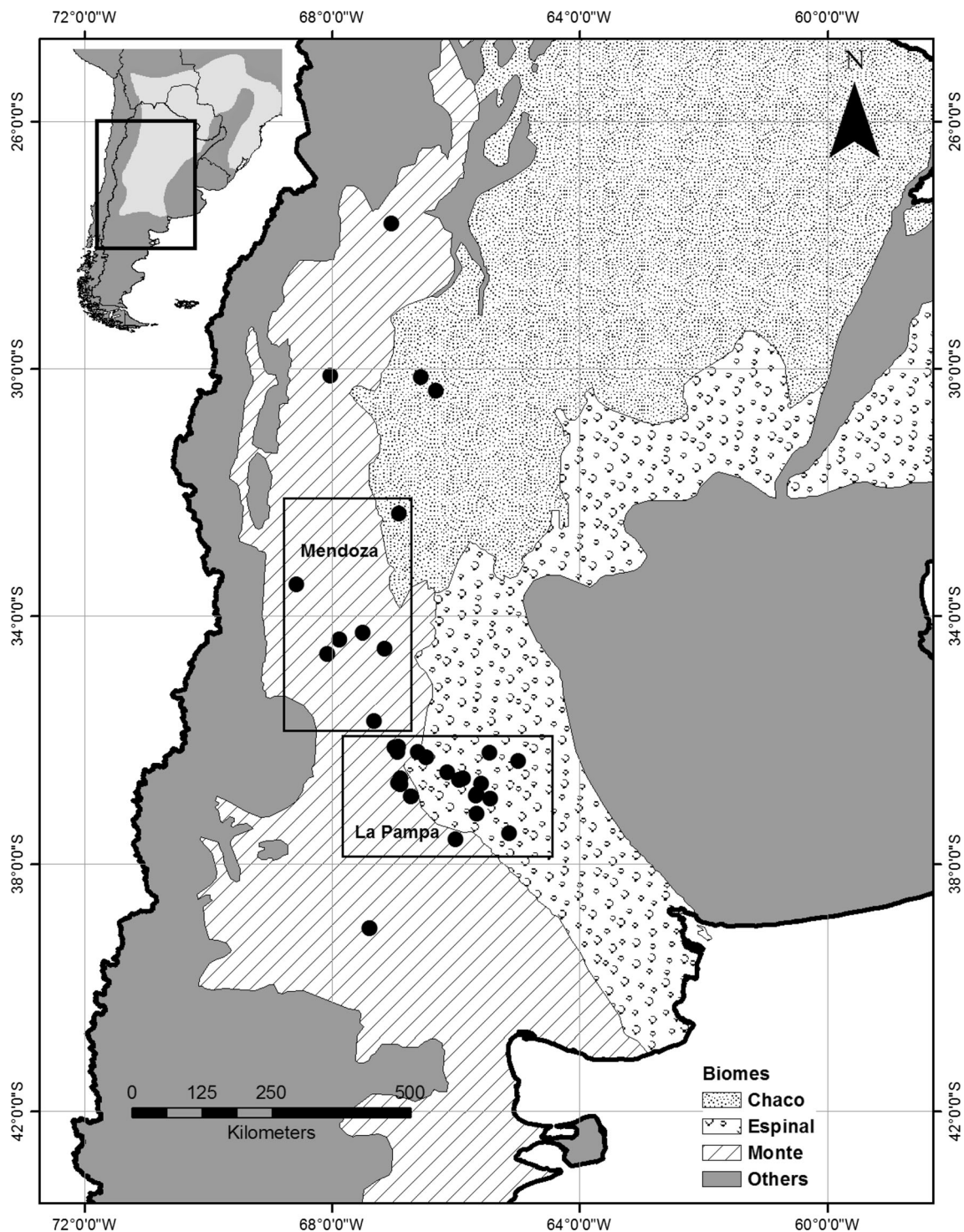
Fig. 1 Distribution of DNA sampling locations of the Crowned Solitary Eagle and extent of the three main semi-arid biomes covered in this study following Cabrera (1976). Polygons indicate populations from the Mendoza and La Pampa areas following the delimitation
