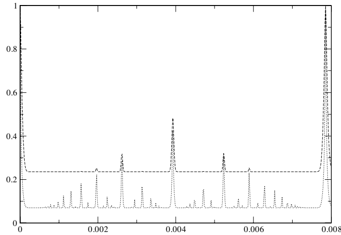
Figure 3. Evolution of \Sigma^{nd}(t) for M = 10^3 , and N = 10 (dashed line) and N = 100 (dotted line), with t_0 = 10^{-3} s.
