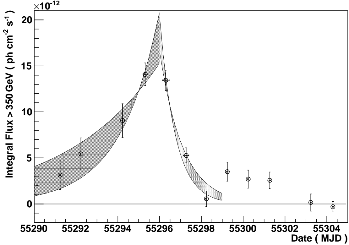
Fig. 3.— Fits to the 2010 April VHE gamma-ray light curve of M87 leading up to the flare and trailing the flare, with fit errors included and shown as shaded regions. The exponential timescale is 2.87^{+1.65}_{-0.99} days for the rising flux portion, and 0.90^{+0.22}_{-0.15} days for MJD 55296–55298 segment of the falling flux.
